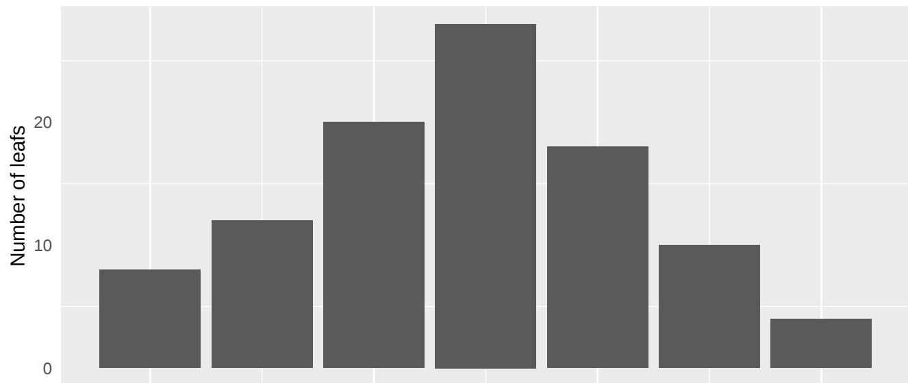
Model complexity
