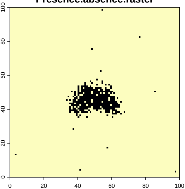
Presence.absence.raster
