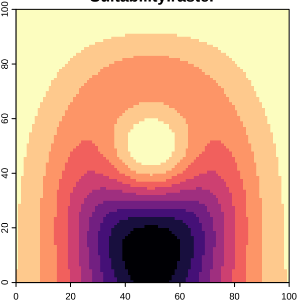
Suitability.raster
