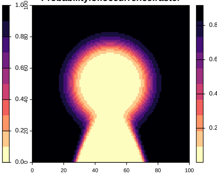
Probability.of.occurrence.raster
