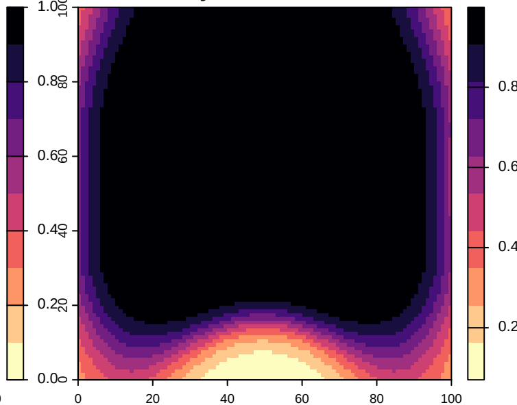
Probability.of.occurrence.raster
