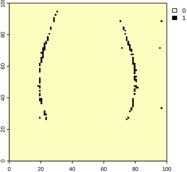
Presence.absence.raster
