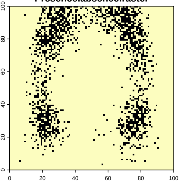
Presence.absence.raster
