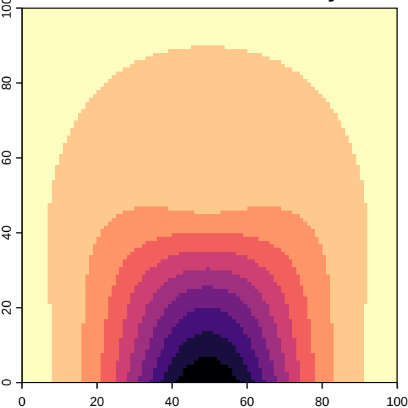
Environmental suitability
