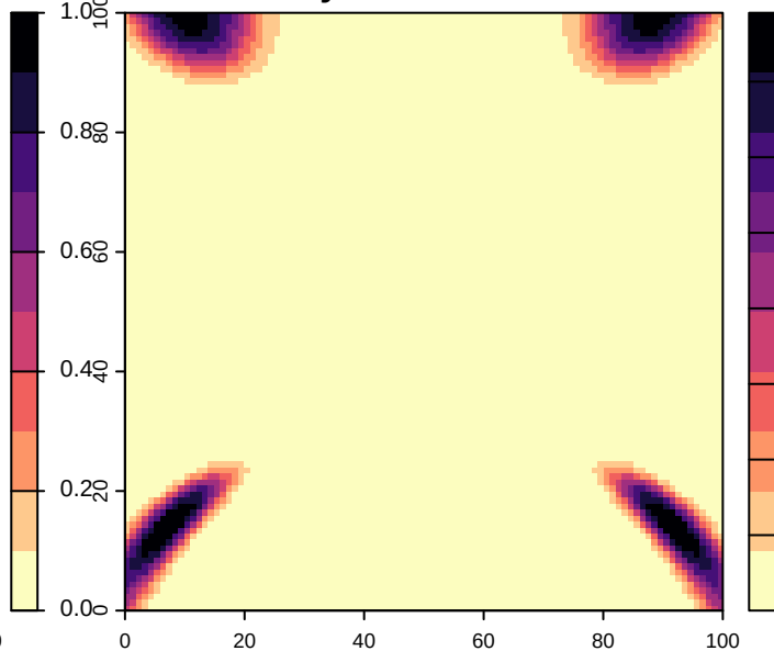
Probability.of.occurrence.raster
