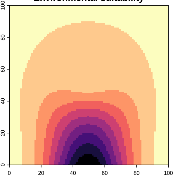
Environmental suitability
