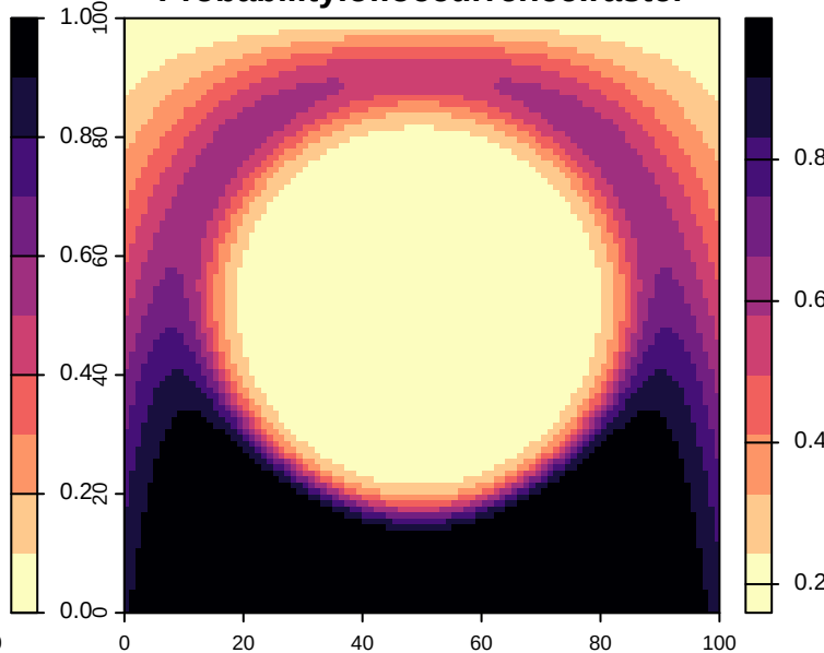
Probability.of.occurrence.raster
