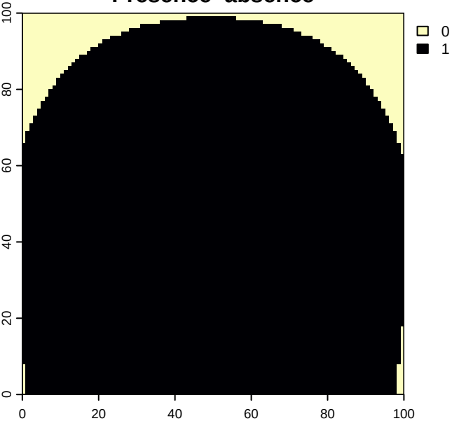
Presence-absence
