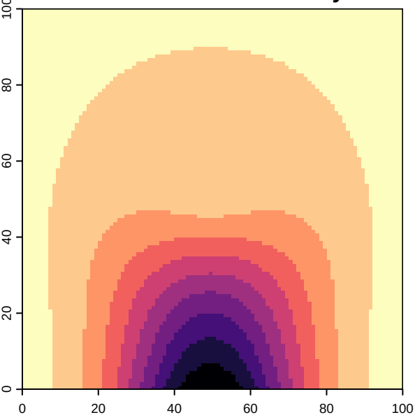
Environmental suitability
