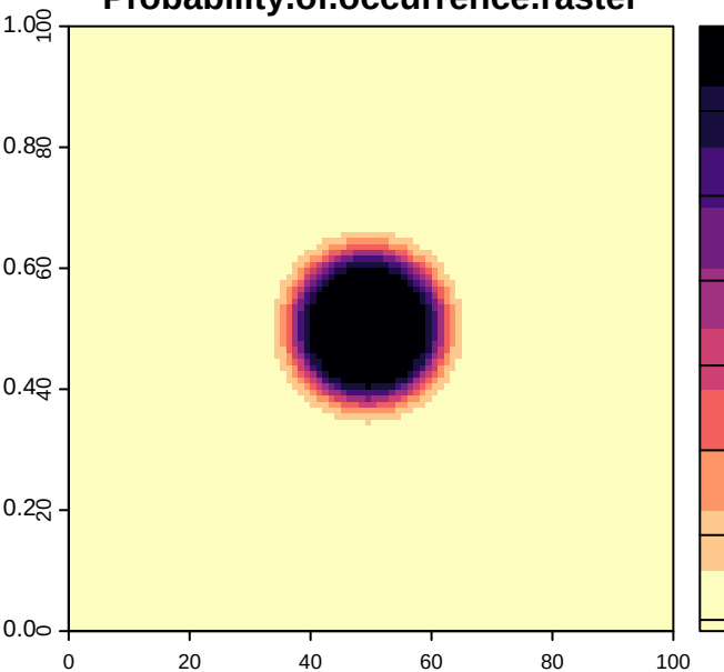
Probability.of.occurrence.raster
