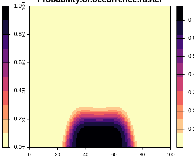
Probability.of.occurrence.raster
