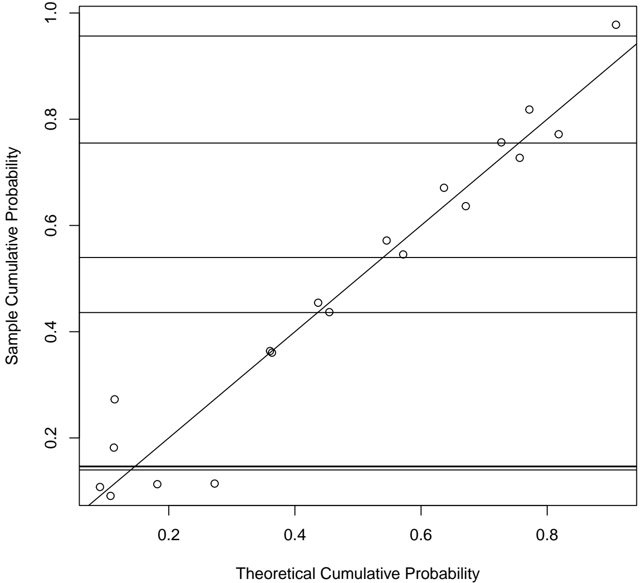
Gamma P-P plot
