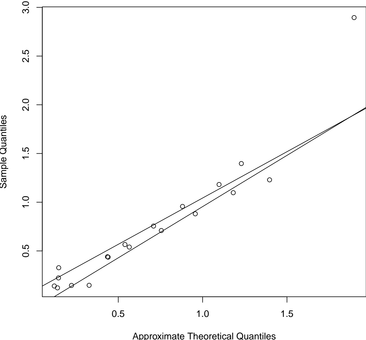
Gamma Q-Q plot
