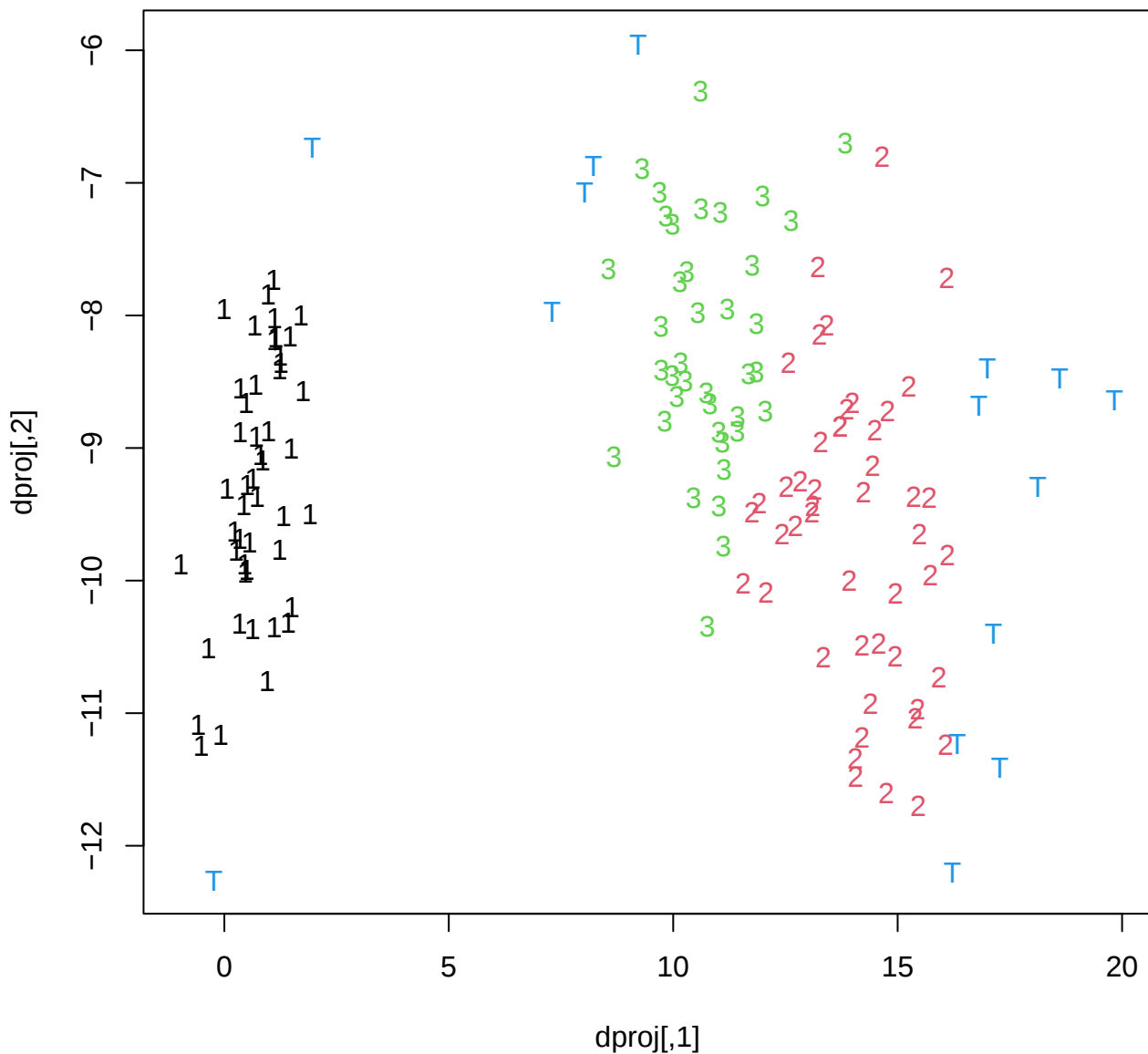
Discriminant coordinates of clusters (T=trimmed)
