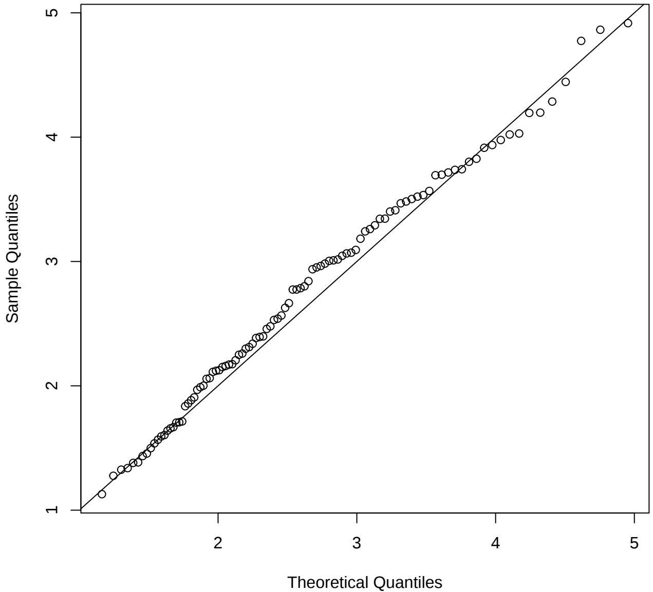
Triangle Q-Q Plot
