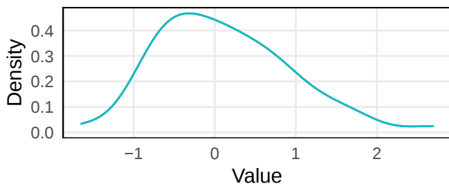
Density Plot: log_c_repulsion
