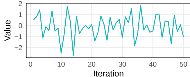
Trace Plot: log_cooling_rate
