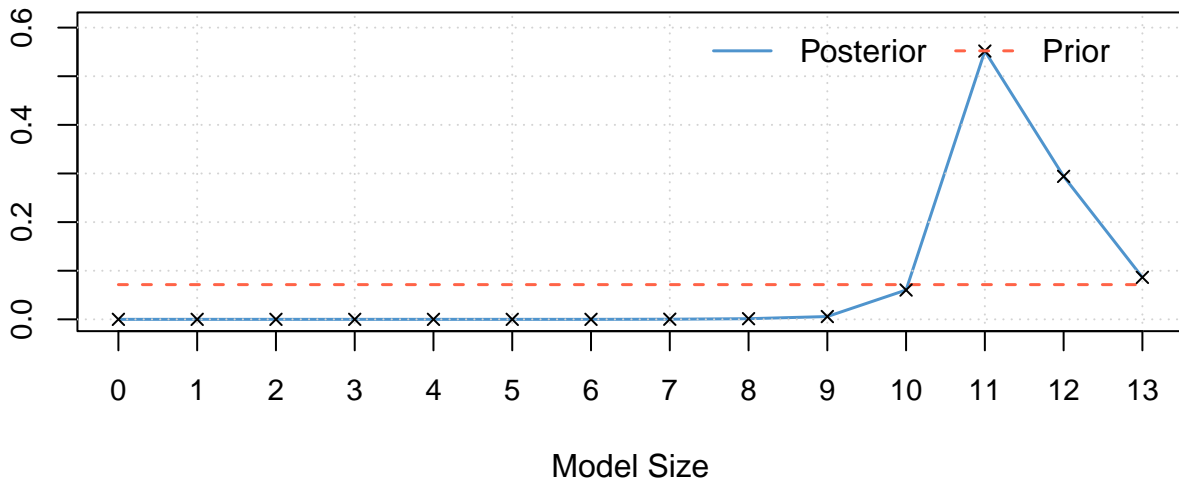
Posterior Model Size Distribution Mean: 11.3898
