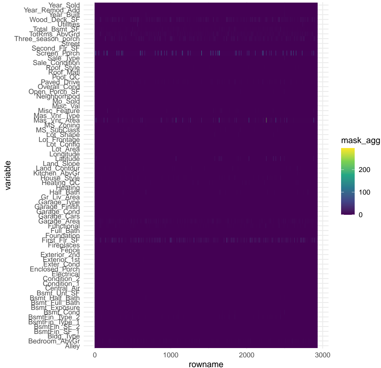
mask_aggregate
