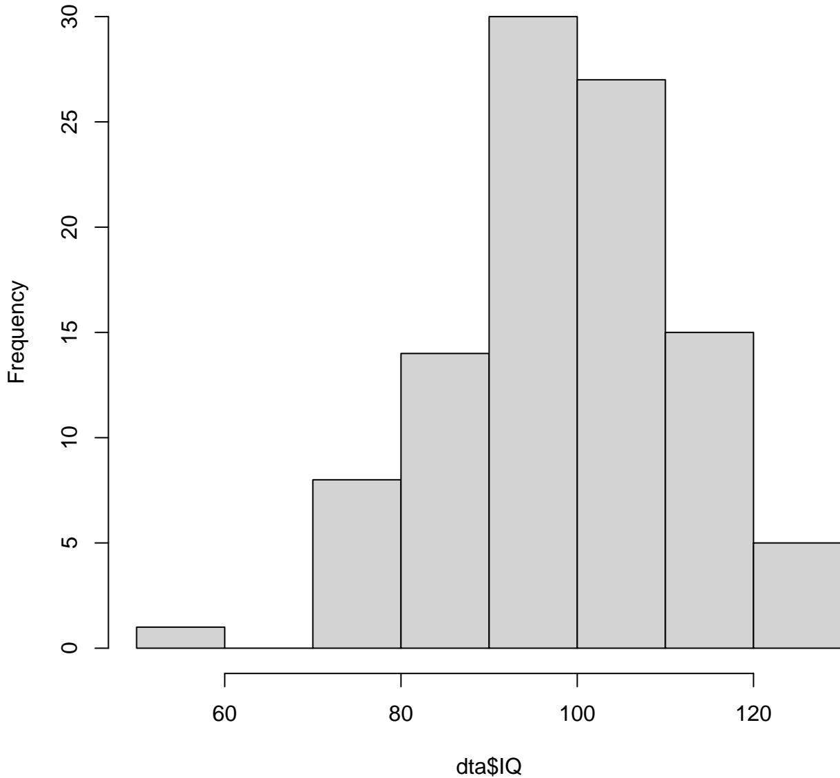
Histogram of dta$IQ
