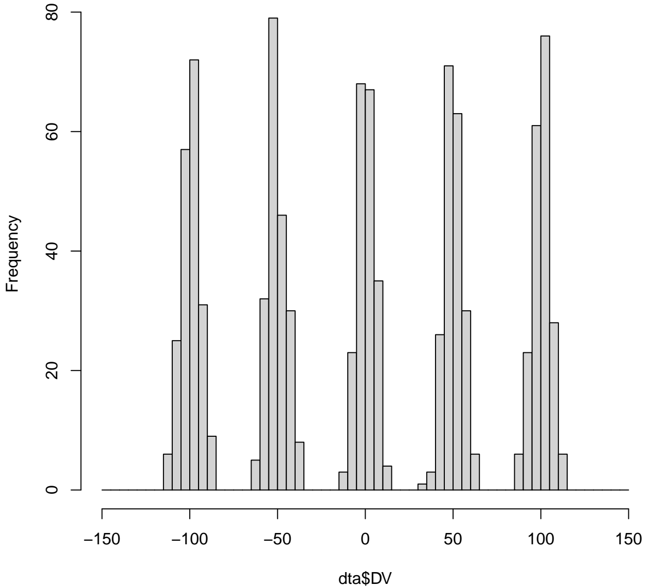
Histogram of dta$DV
