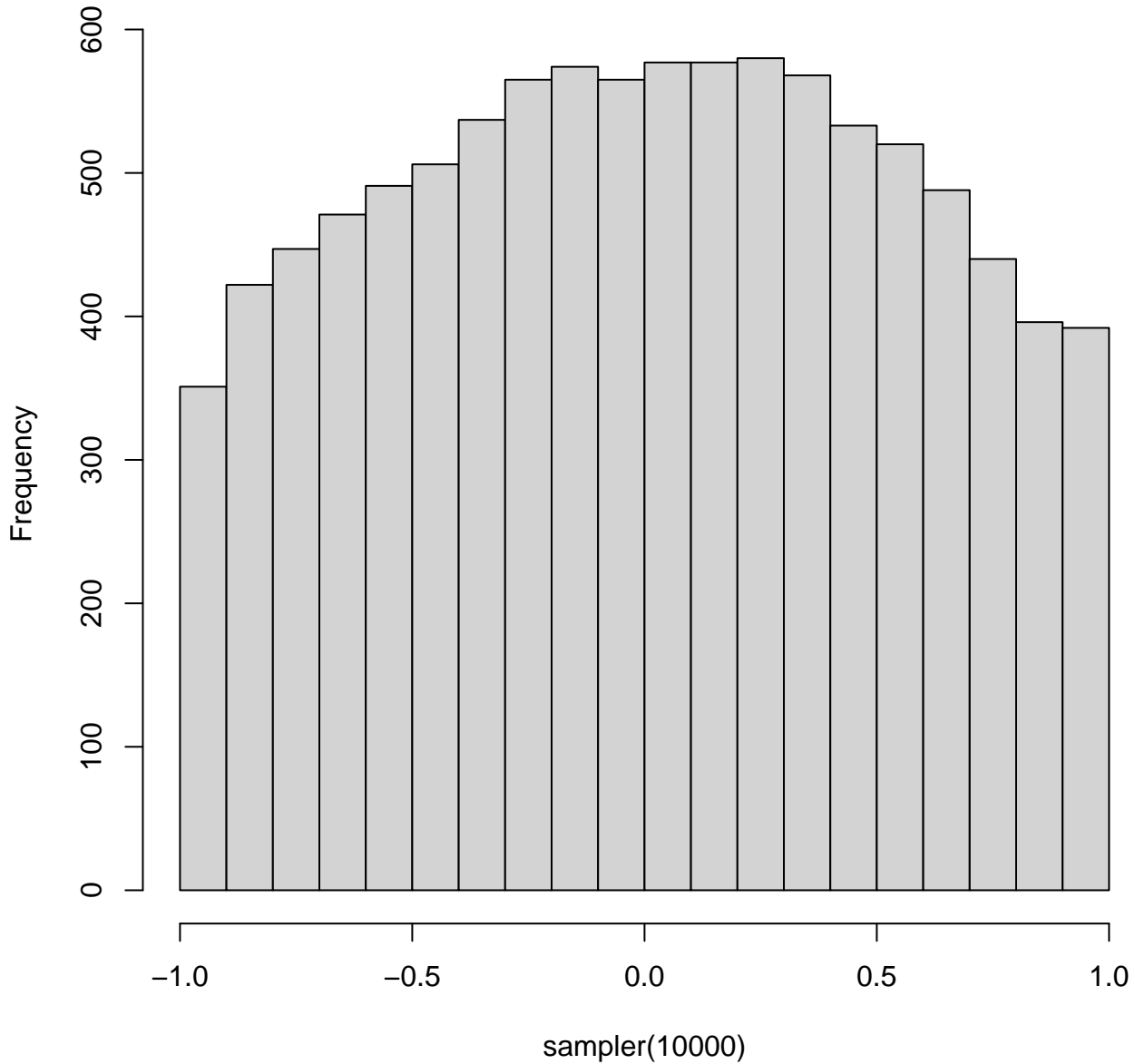
Histogram of sampler(10000)
