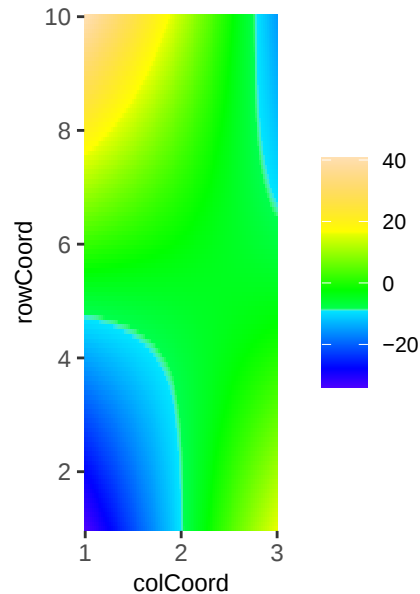
Fitted Spatial Trend
