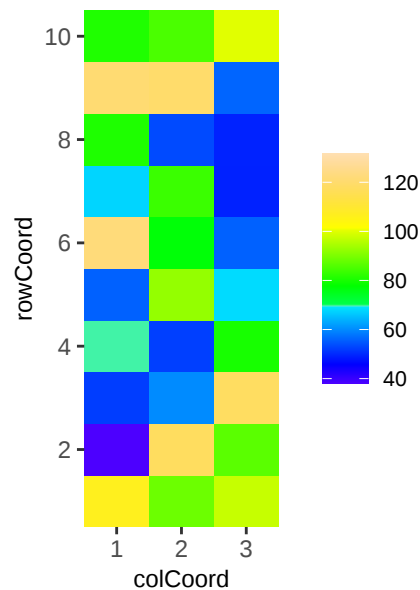
Fitted Spatial Trend
