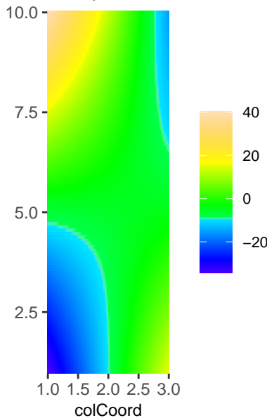
Fitted Spatial Trend
