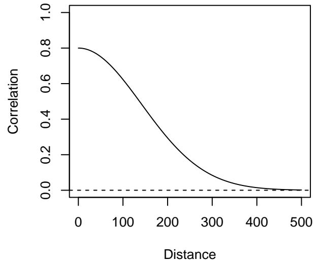
'Gaussian', acf0 = 0.8, range = 200
