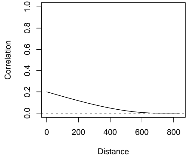
'Spherical', acf0 = 0.2, range = 700
