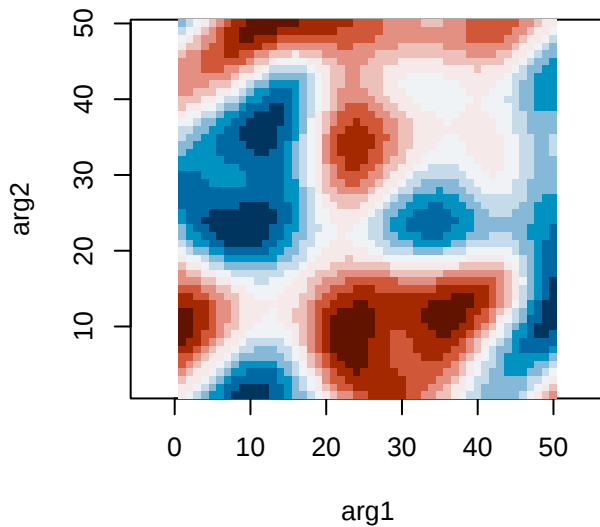
Skew-symmetric part of y
