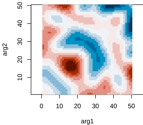
Symmetric part of y
