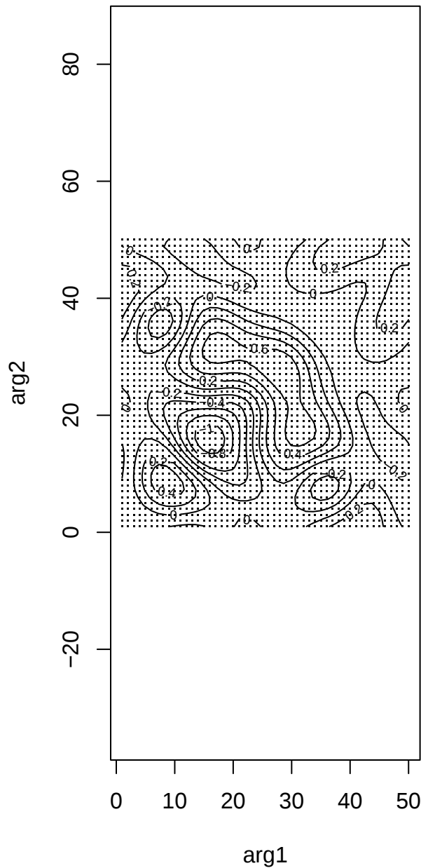
s(\arg1, \arg2, 26.6)
