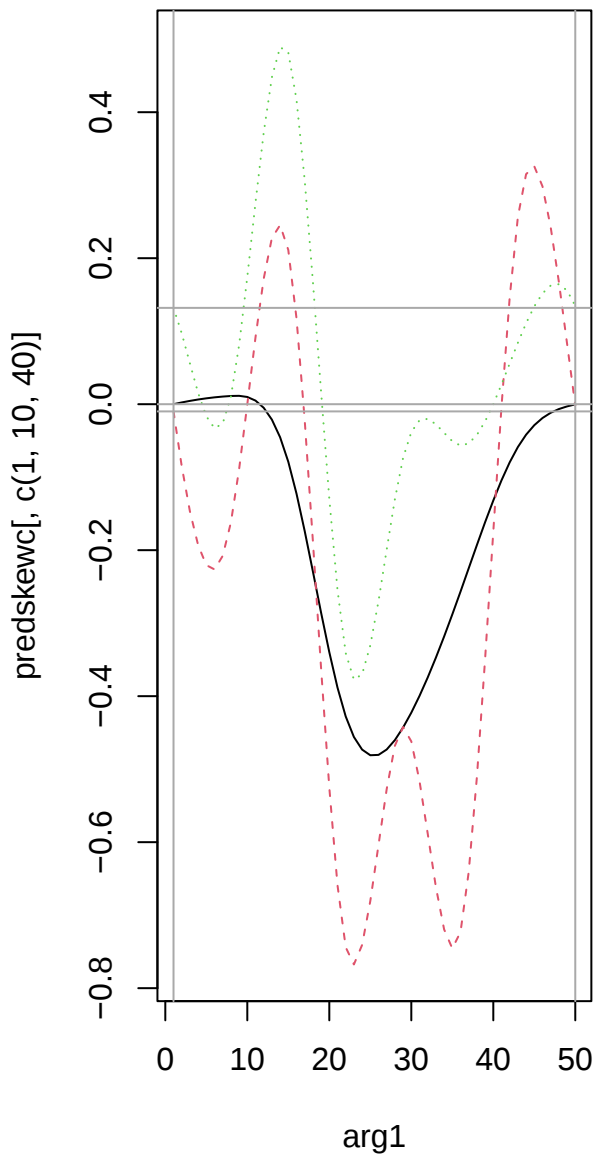
skew-symmetric smooth
