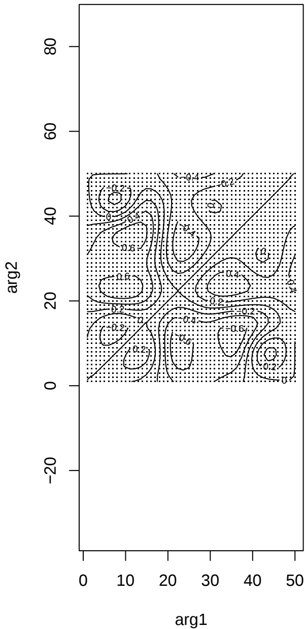
s(\arg1, \arg2, 20.95)
