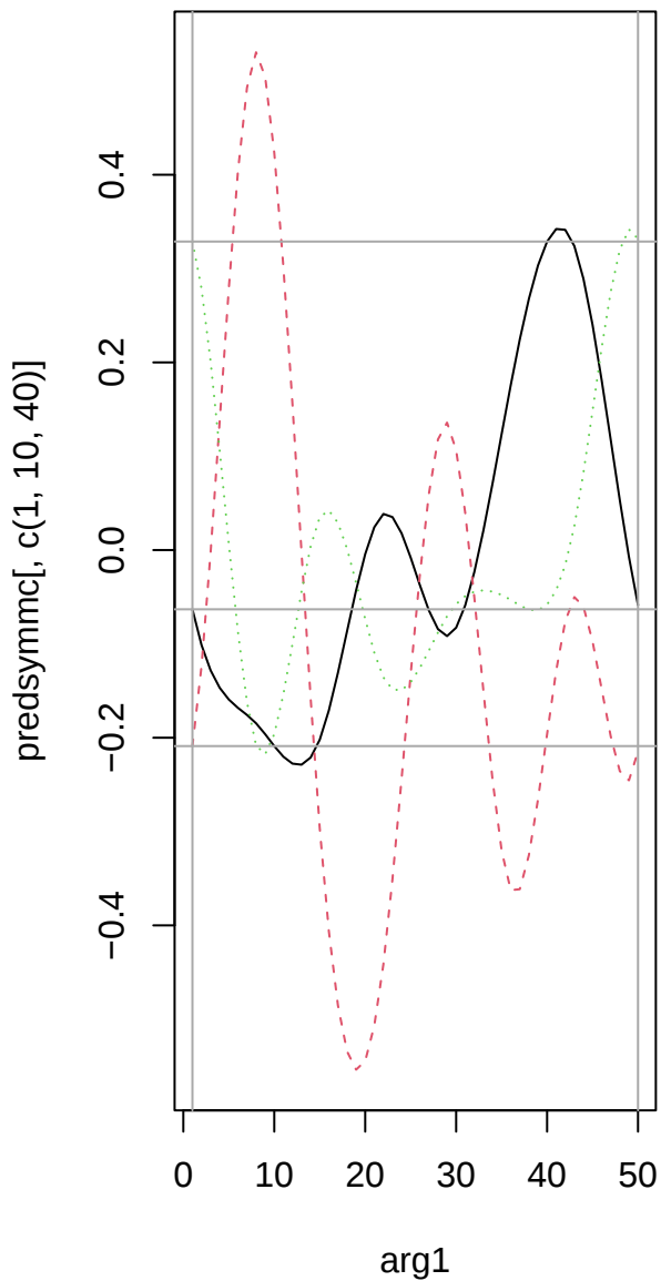
symmetric smooth
