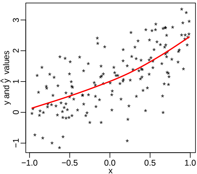
Convex Regression using Penalized Least Squares ( \lambda=0.5 )
