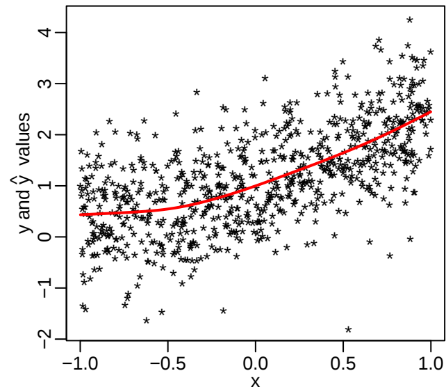
Convex Regression using Penalized Least Squares ( \lambda=0.5 )
