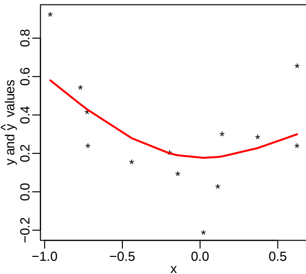
Convex Regression using Penalized Least Squares ( \lambda=0.2 )
