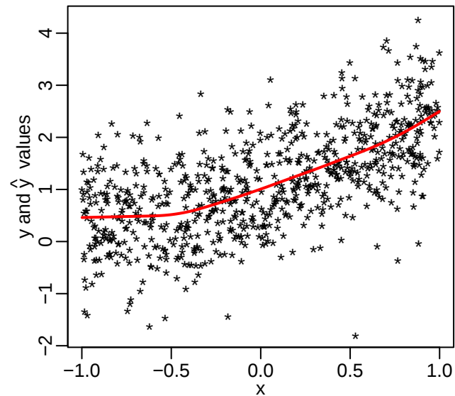
Convex Regression using Penalized Least Squares ( \lambda=0.1 )
