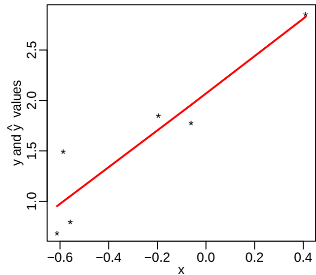
Convex Regression using Penalized Least Squares (lambda=0.1)
