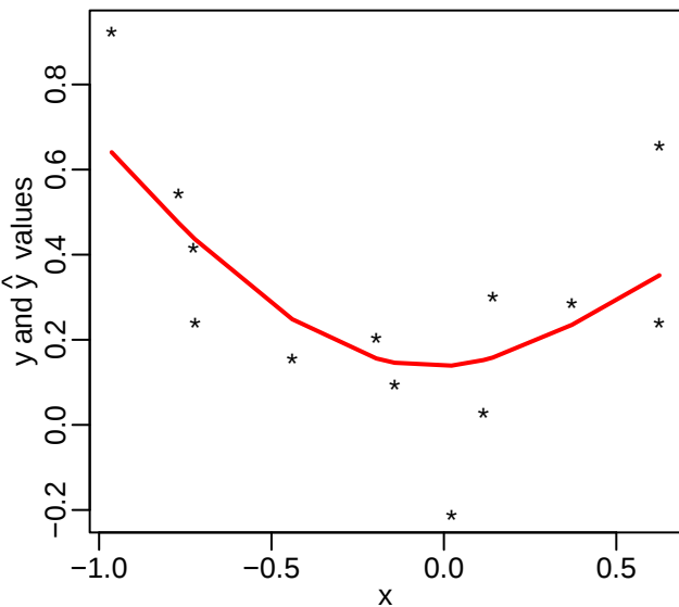
Convex Regression using Penalized Least Squares ( \lambda=0.1 )
