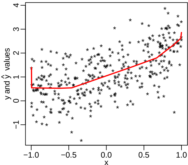
Convex Regression using Least Squares
