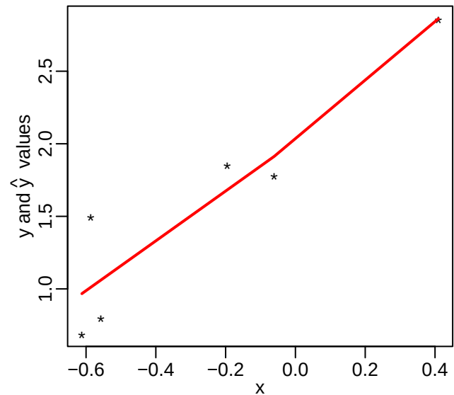
Convex Regression using Least Squares
