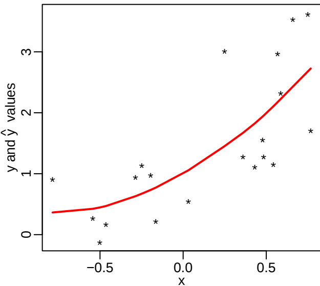
Smoothing Spline using Penalized Least Squares
