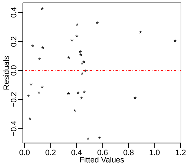
Fitted vs Residuals
