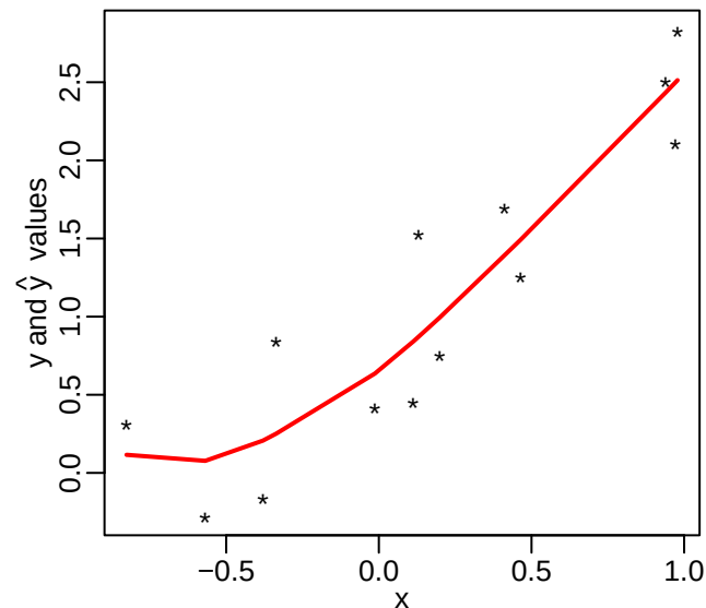
Smoothing Spline using Penalized Least Squares
