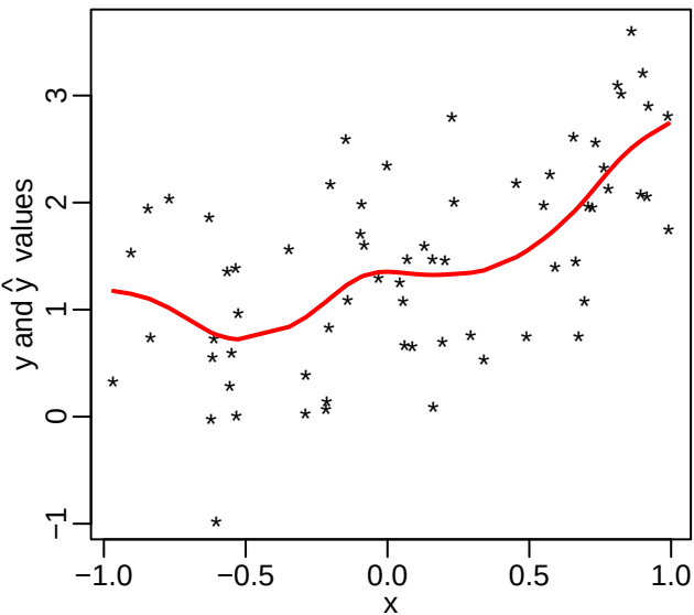
Smoothing Spline using Penalized Least Squares
