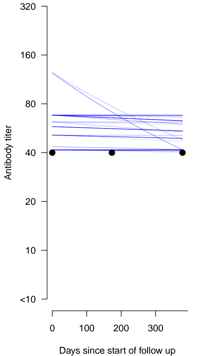
Individual 50 P(infection) = 0.00
