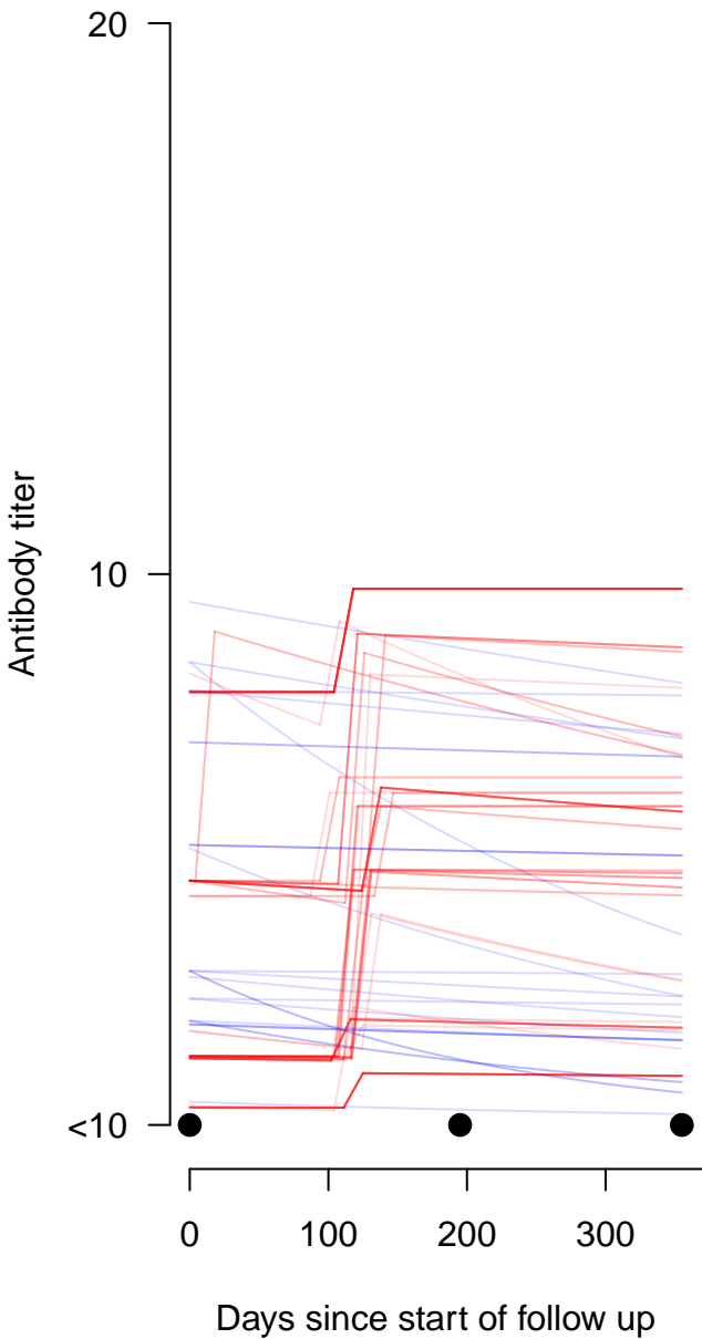
Individual 1 P(infection) = 0.75
