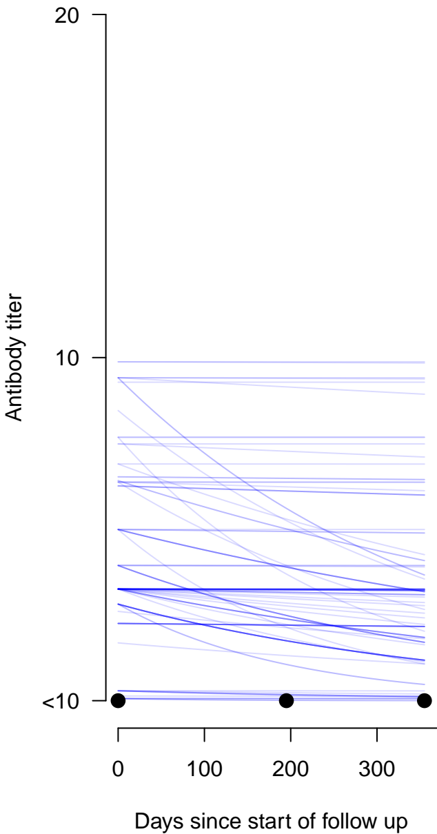
Individual 1 P(infection) = 0.00
