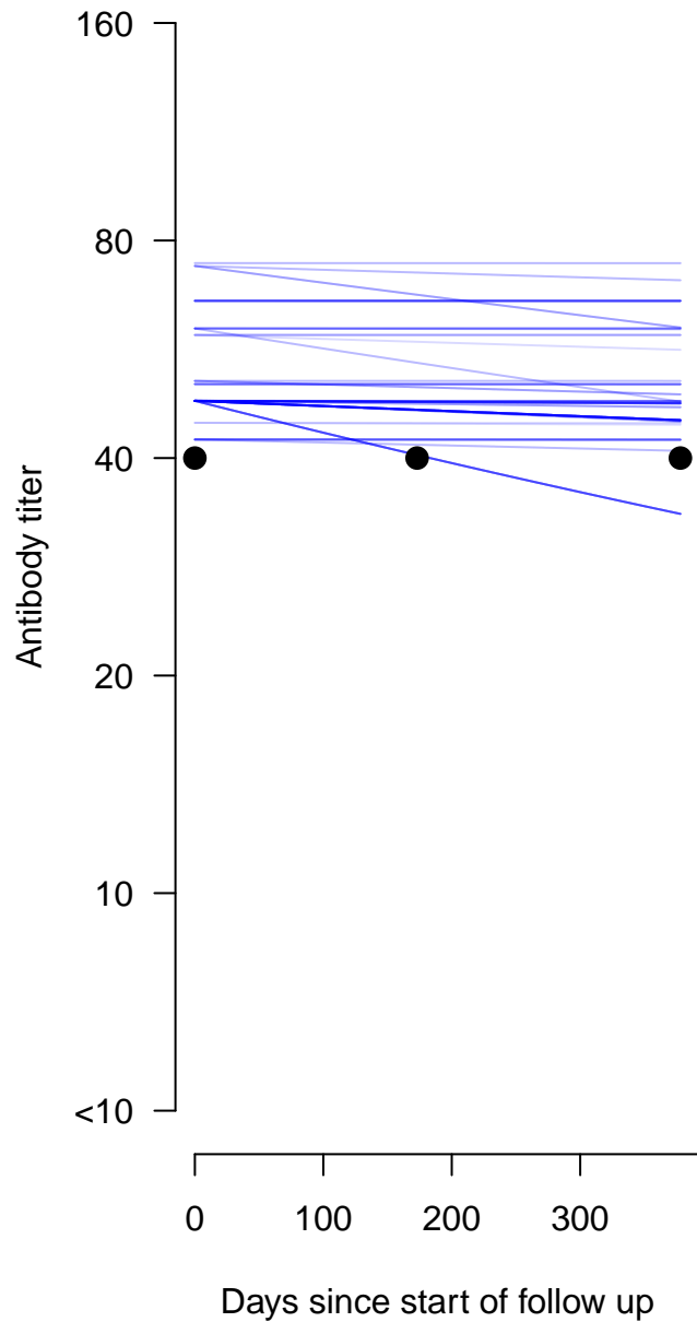
Individual 50 P(infection) = 0.00
