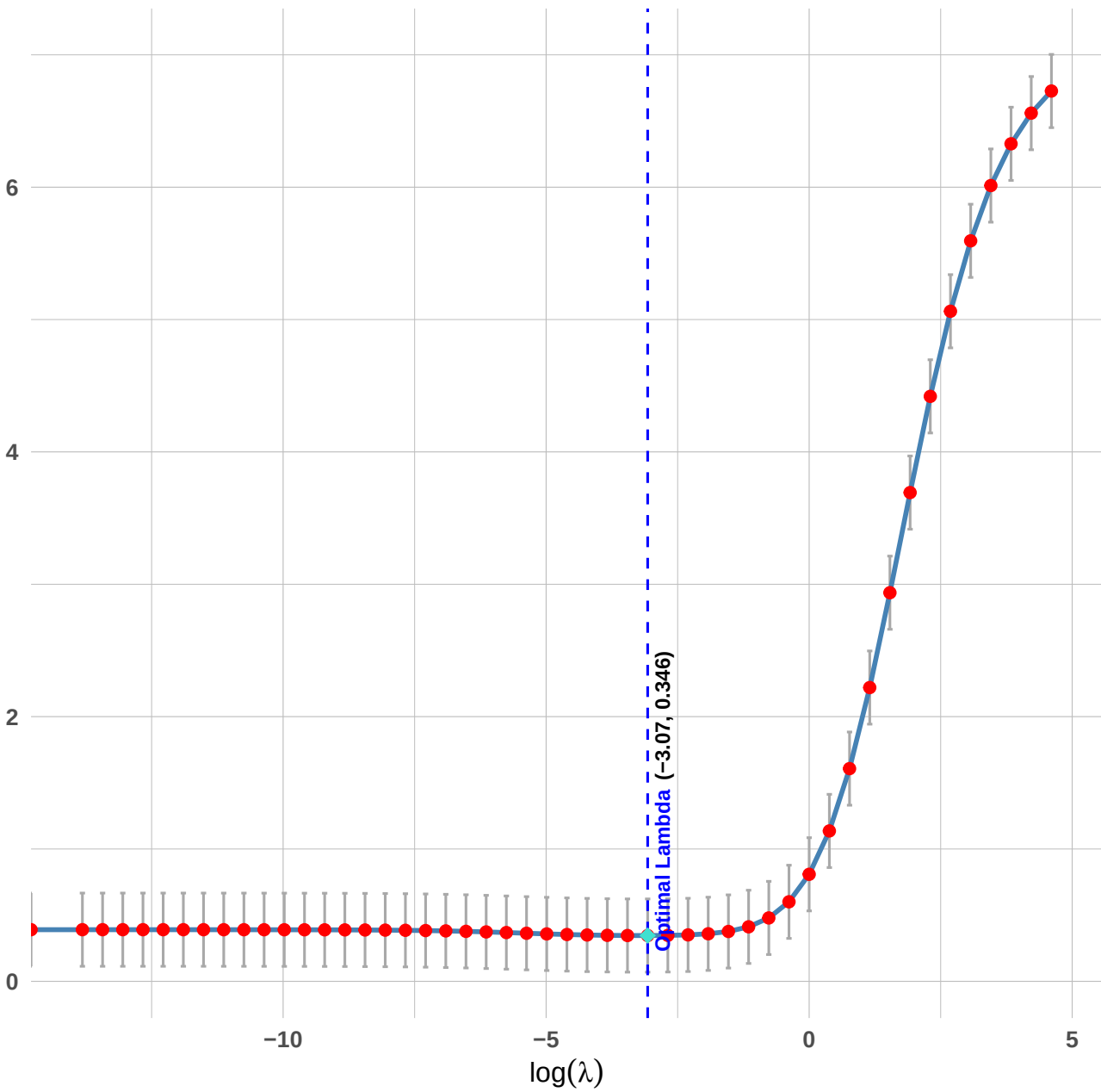
Cross-Validation Curve
