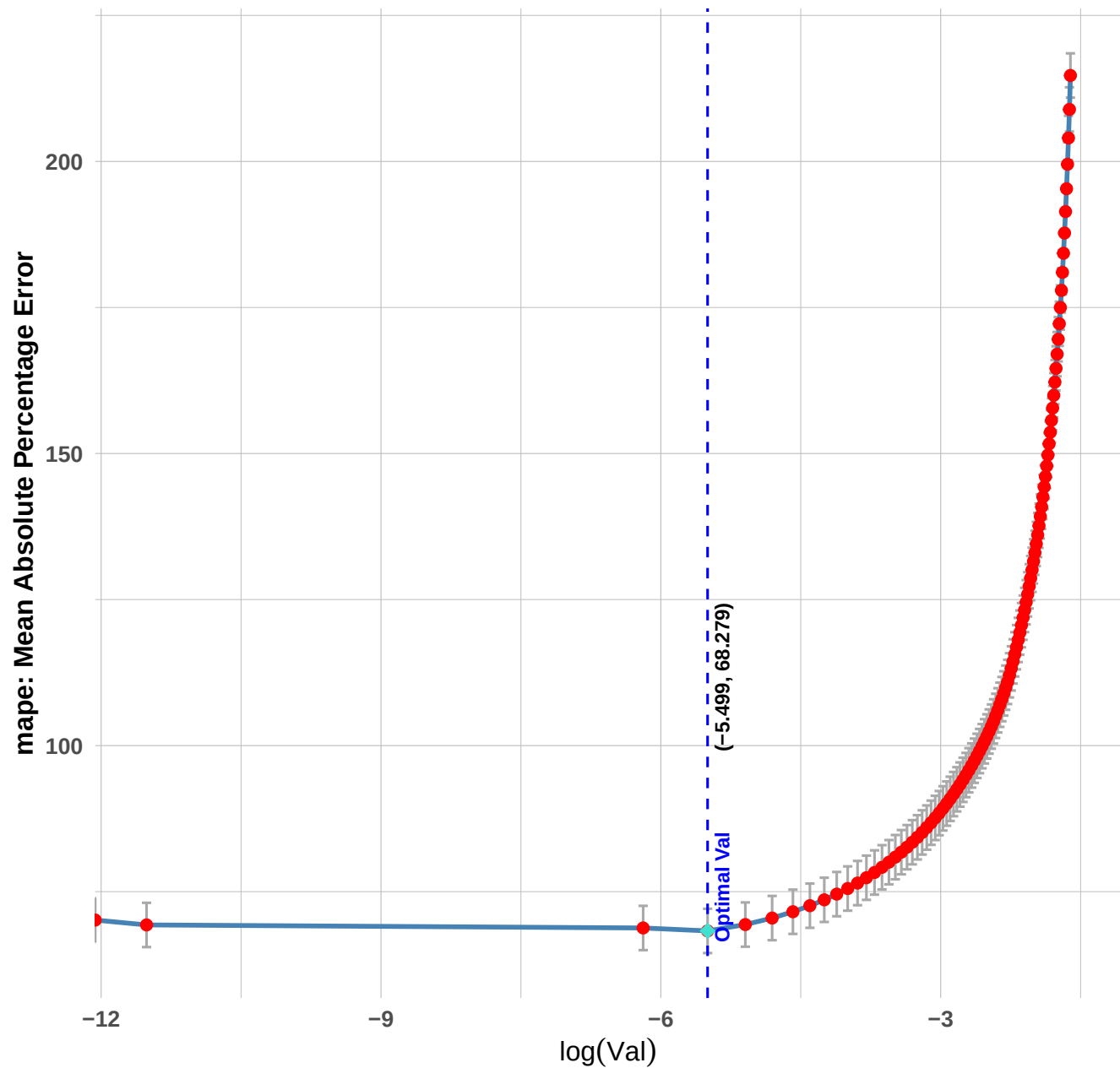
Cross-Validation Curve
