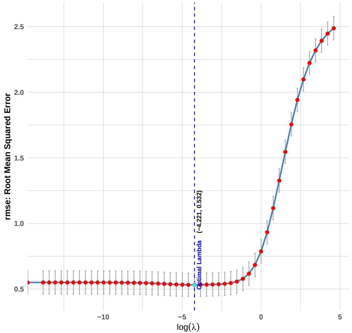
Cross-Validation Curve
