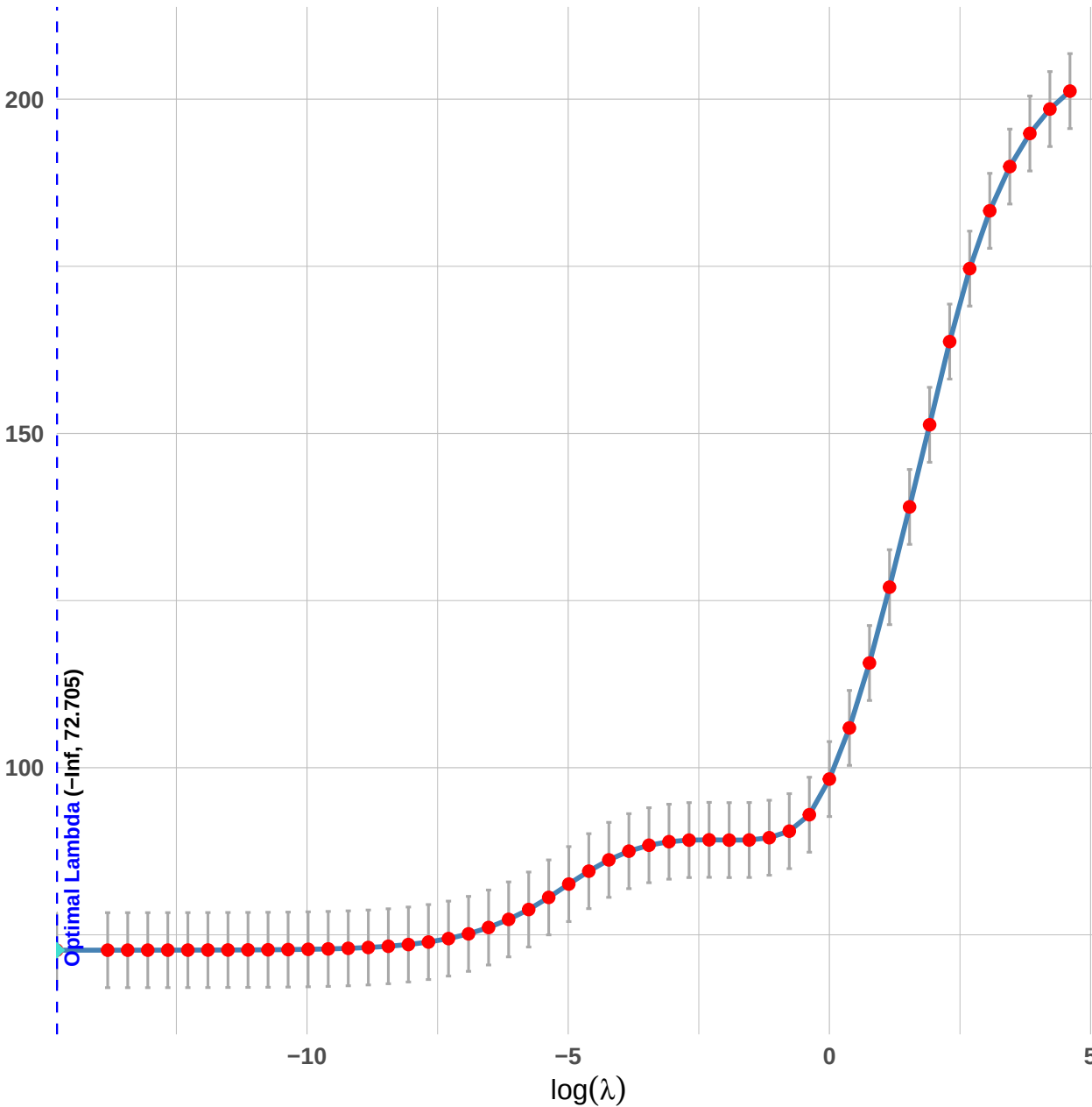
Cross-Validation Curve
