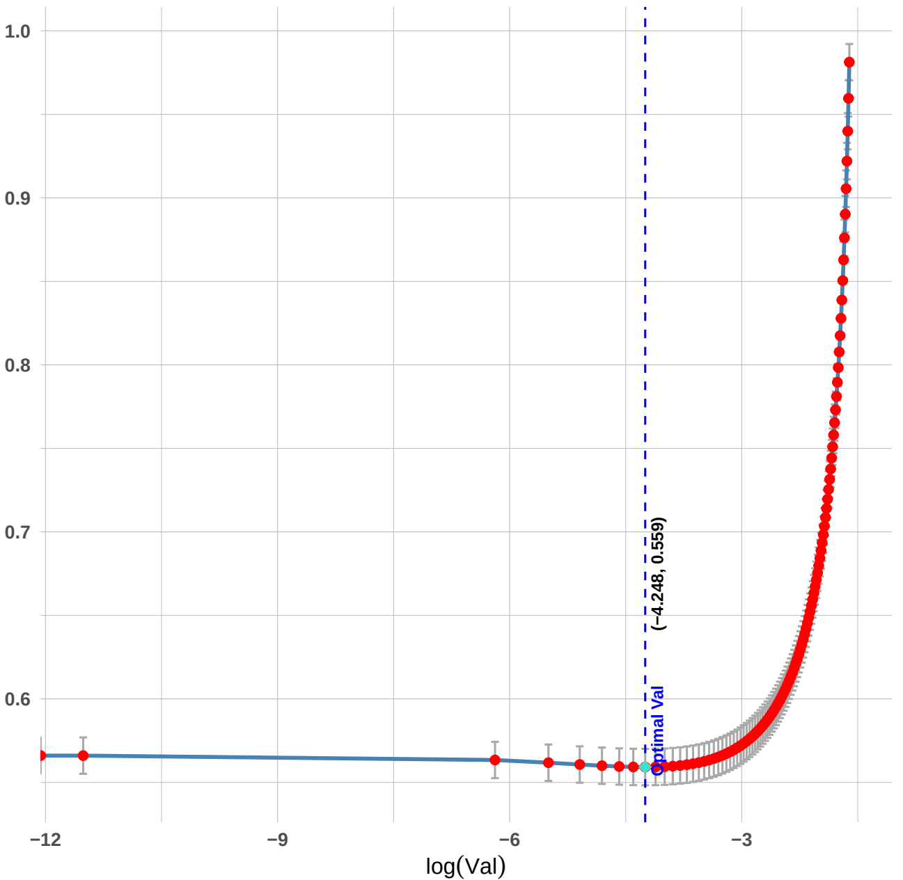
Cross-Validation Curve
