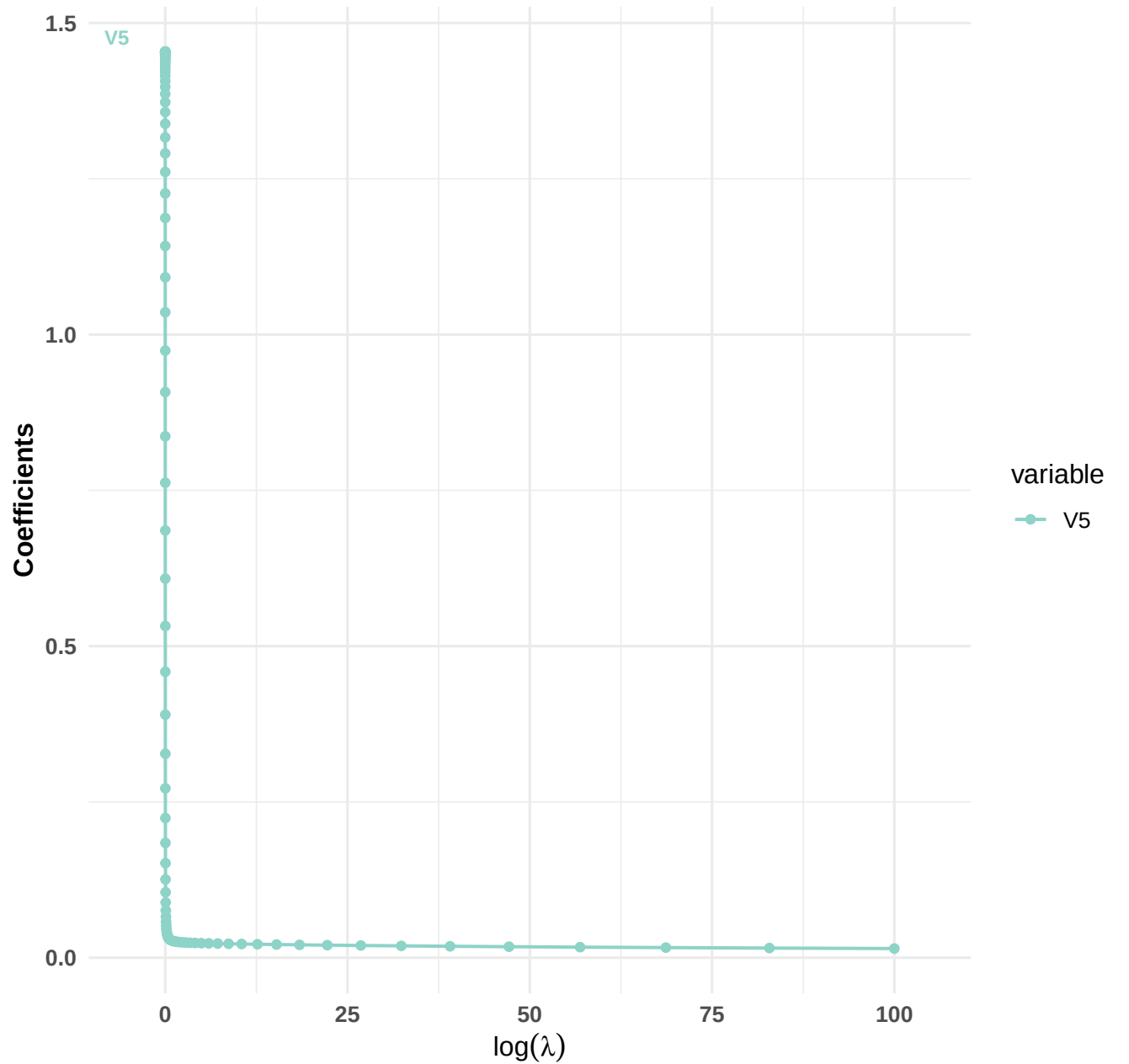
Coefficient Profile Plot (Variables 6 to 6 )
