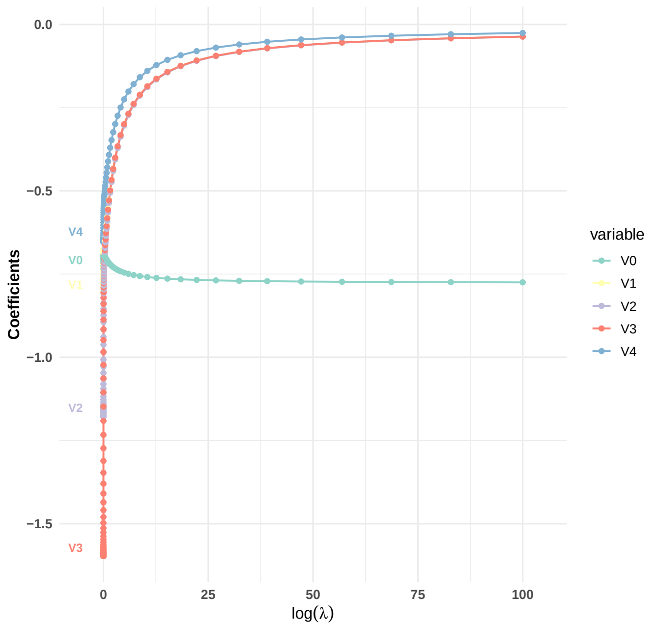
Coefficient Profile Plot (Variables 1 to 5 )
