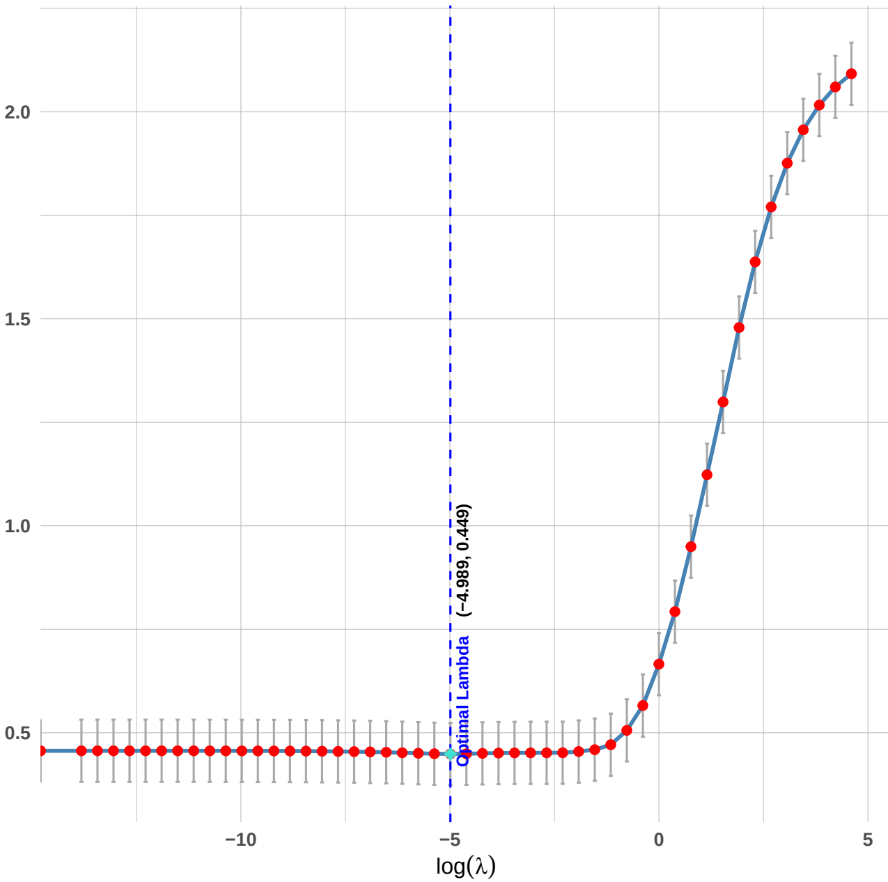
Cross-Validation Curve
