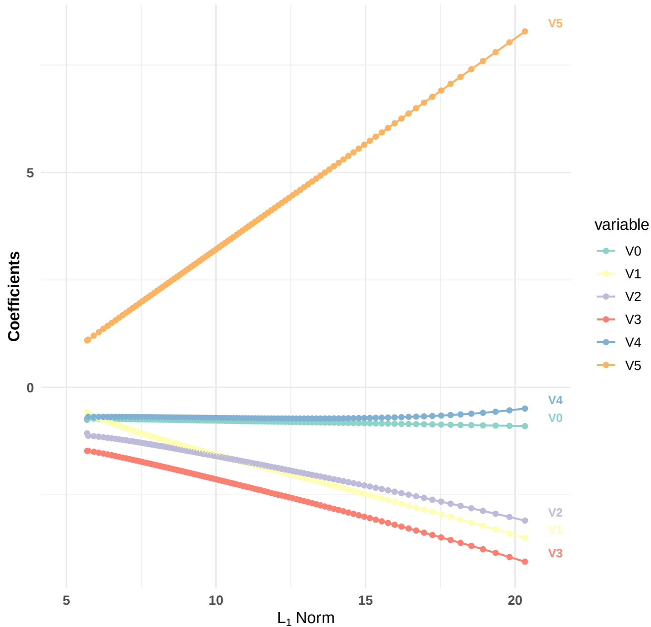
Coefficient Profile Plot (Variables 1 to 6 )
