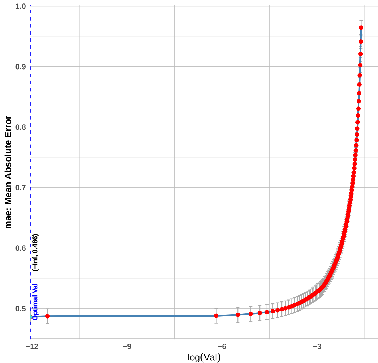
Cross-Validation Curve
