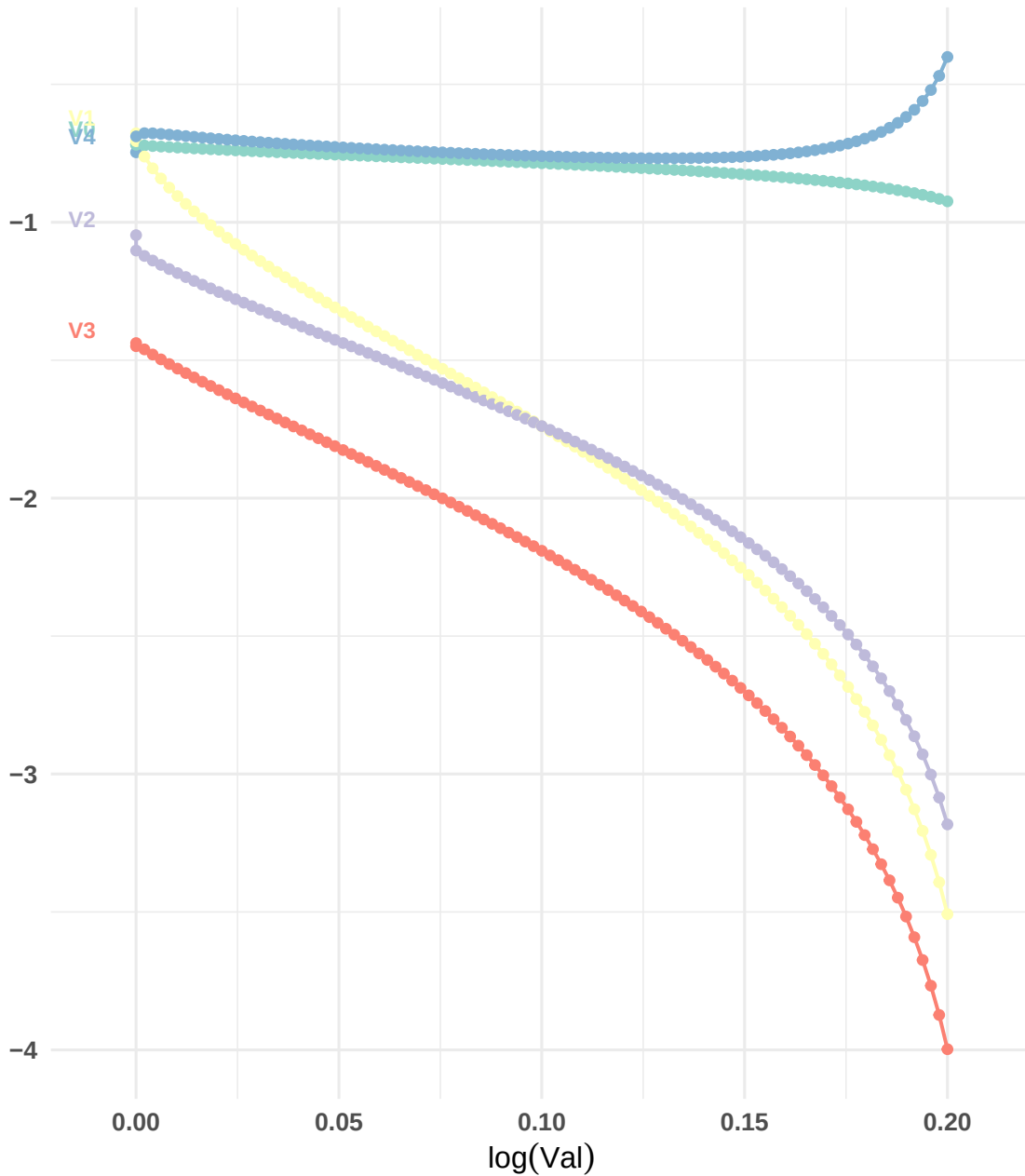
Coefficient Profile Plot (Variables 1 to 5 )
