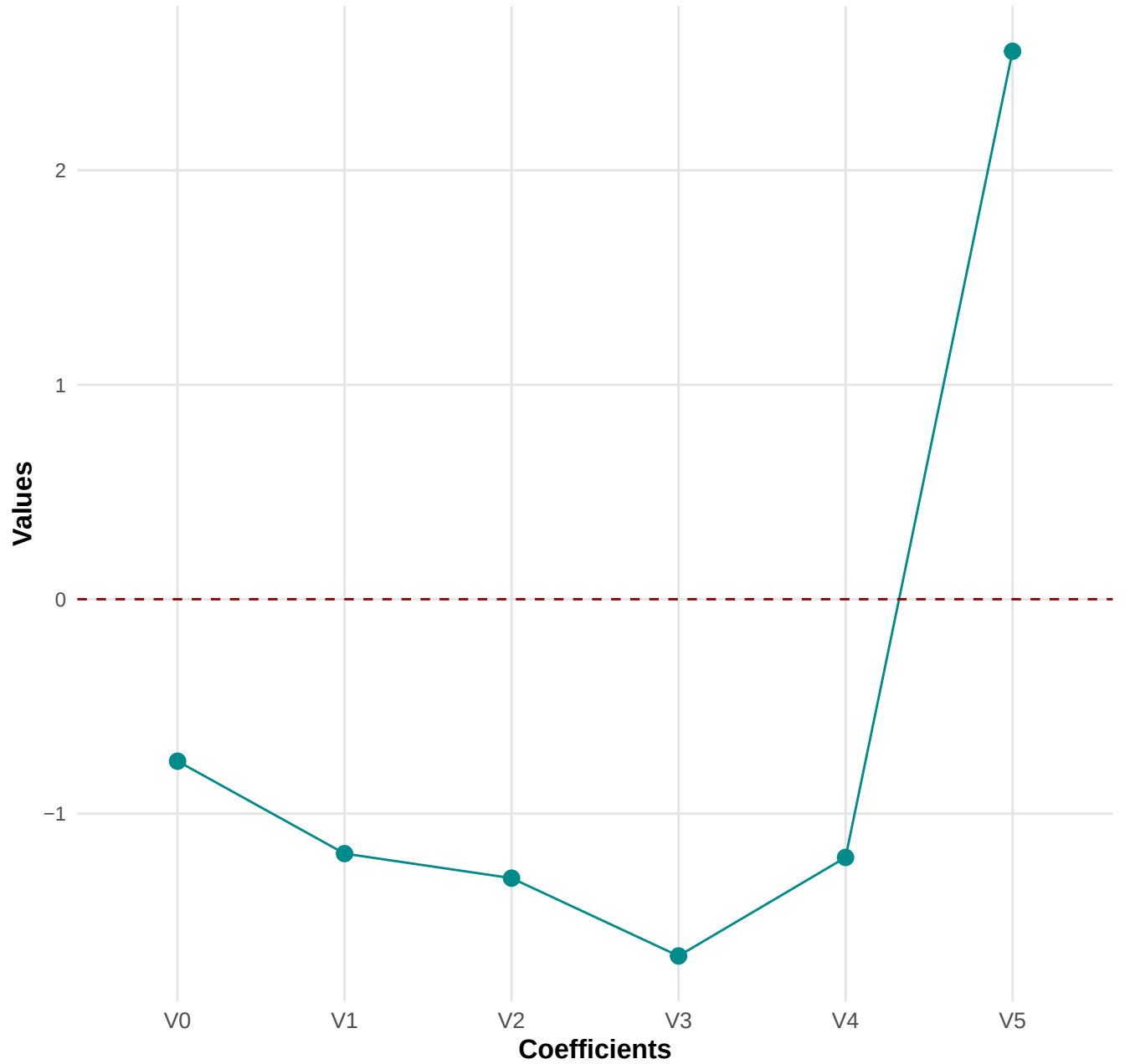
Estimated Coefficients
