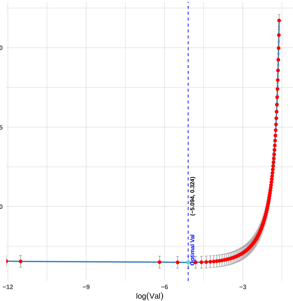
Cross-Validation Curve
