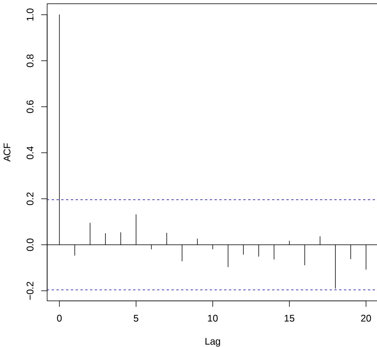
Series ts1
