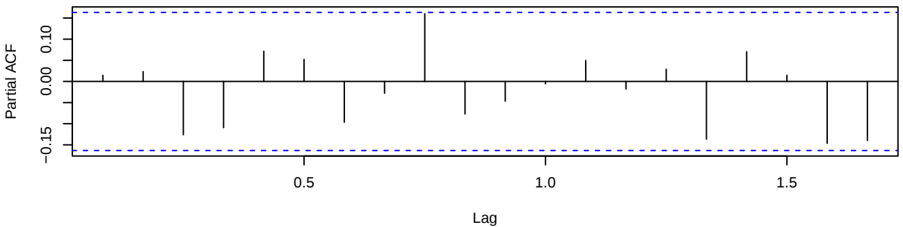
PACF of Residuals
