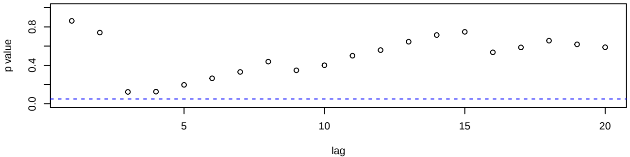
p values for Box-Pierce statistic
