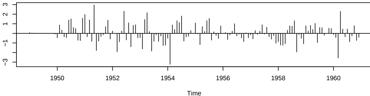
Standardized Residuals
