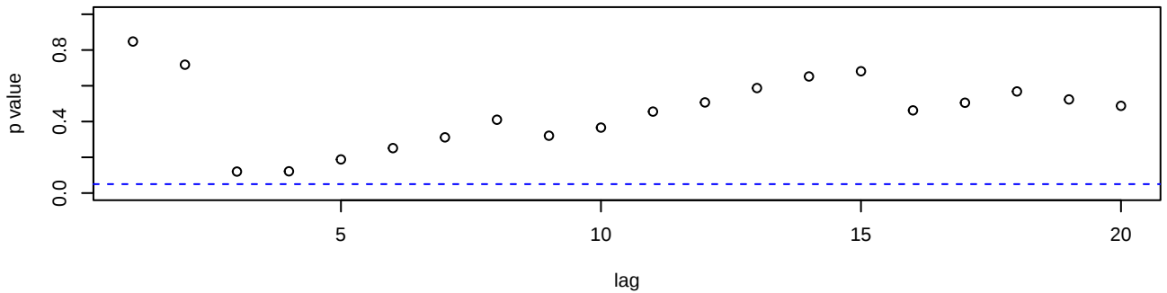
p values for Li-McLeod statistic
