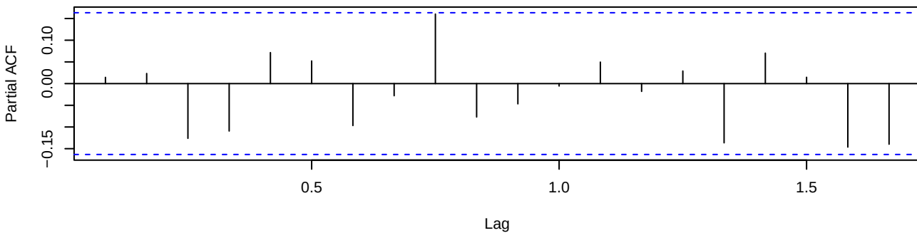
PACF of Residuals
