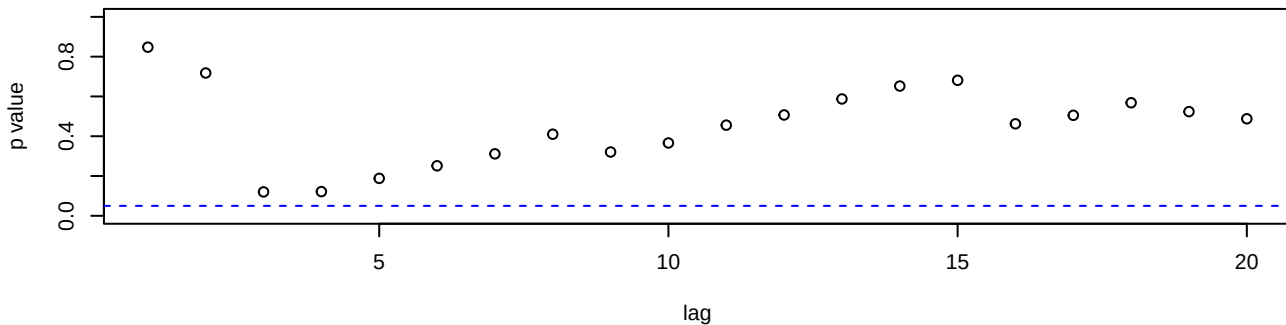
p values for Li-McLeod statistic
