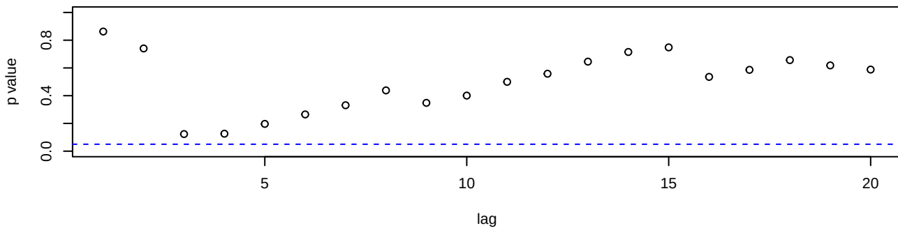
p values for Box-Pierce statistic
