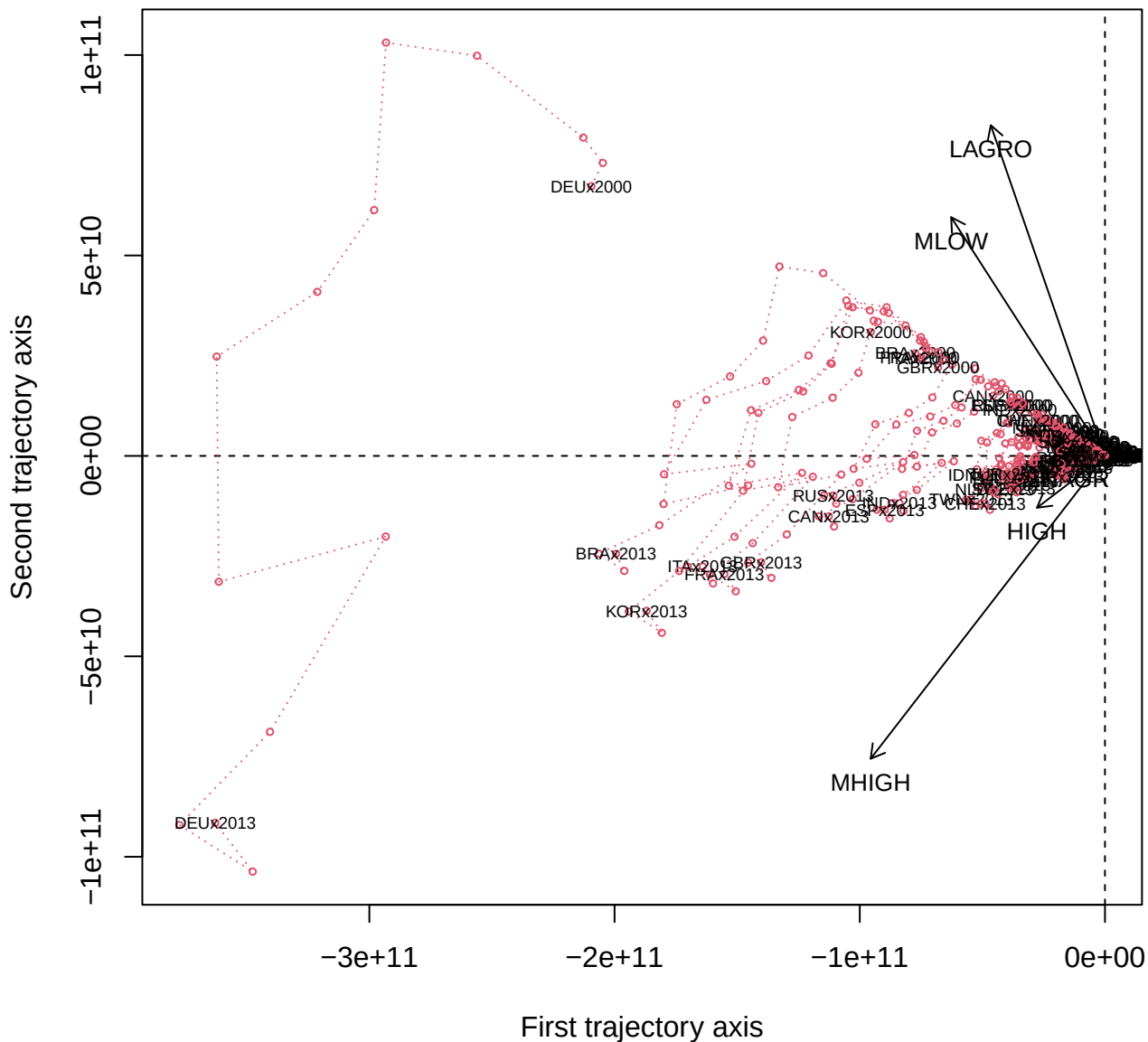
Trajectory biplot
