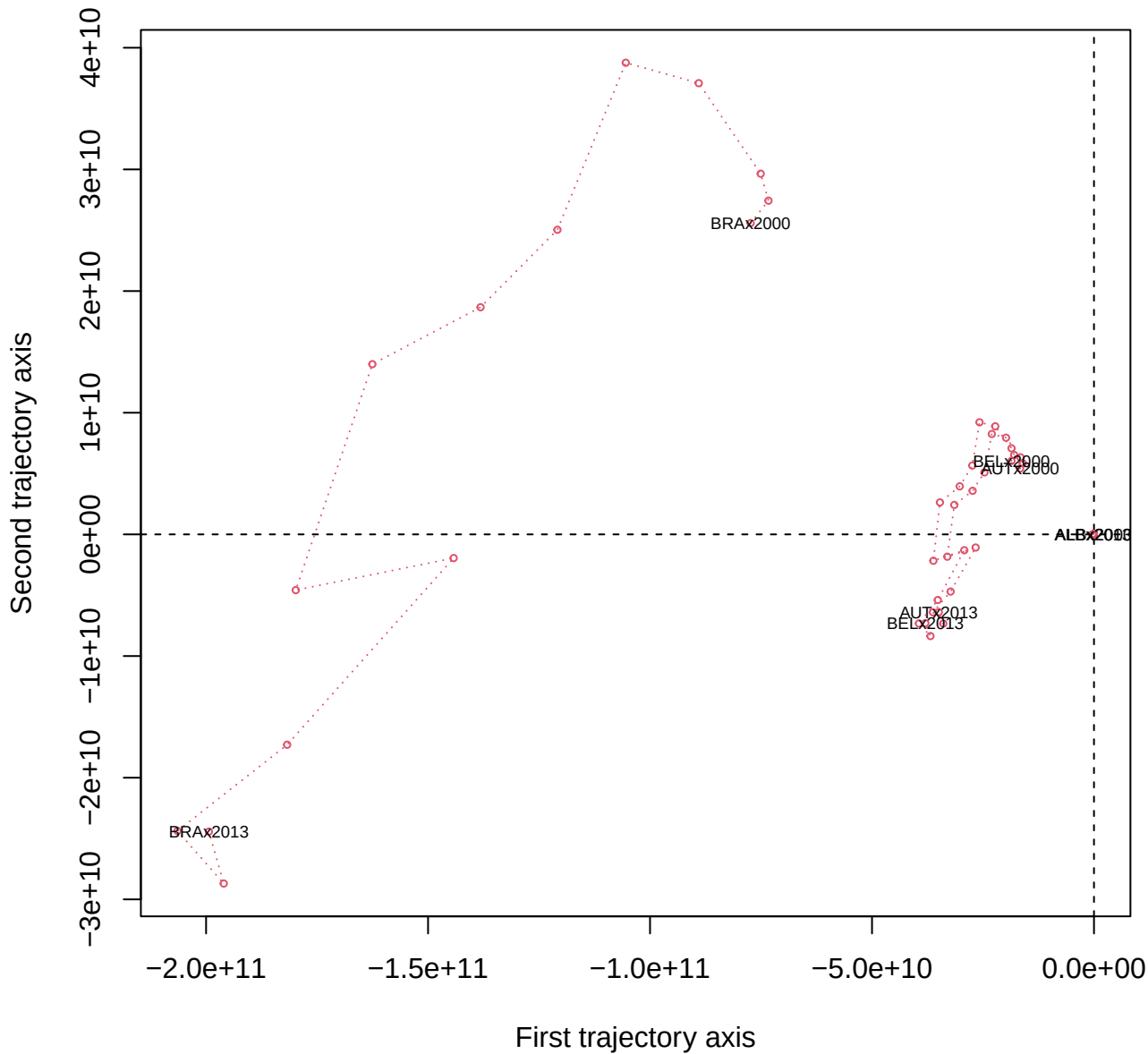
Trajectory biplot
