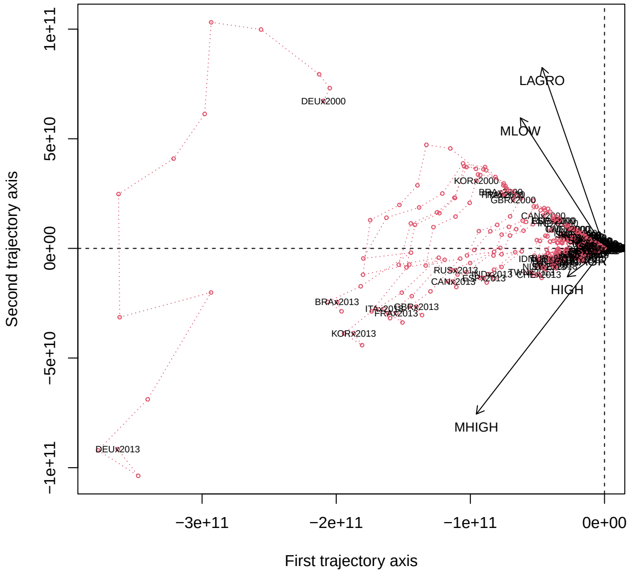
Trajectory biplot
