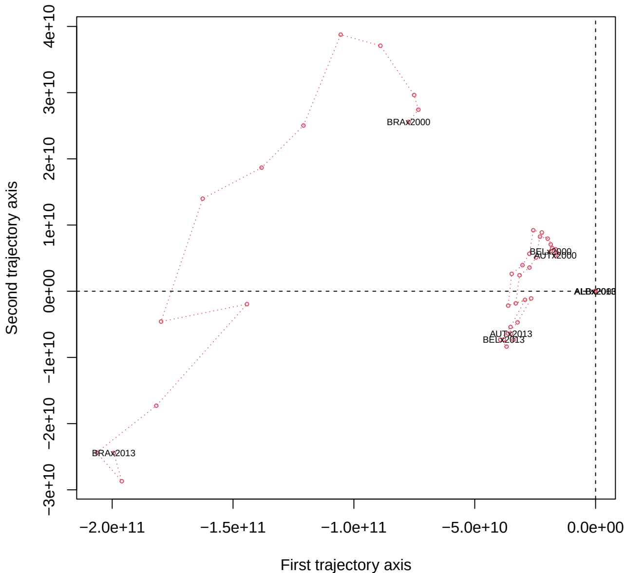
Trajectory biplot
