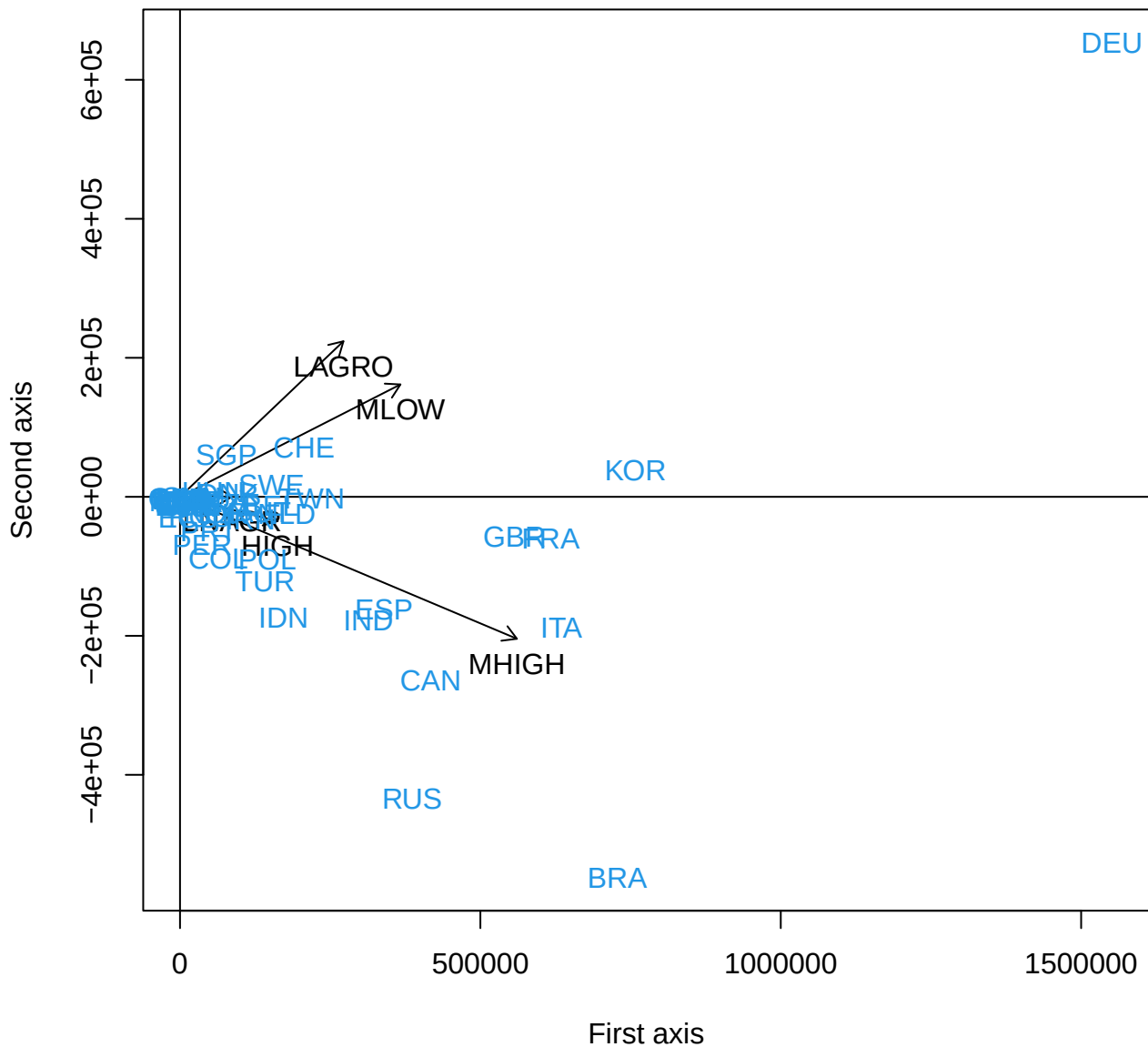
Joint biplot
