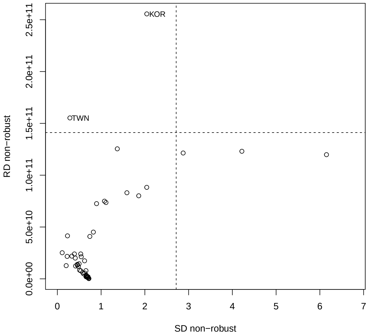
Distance-distance plot
