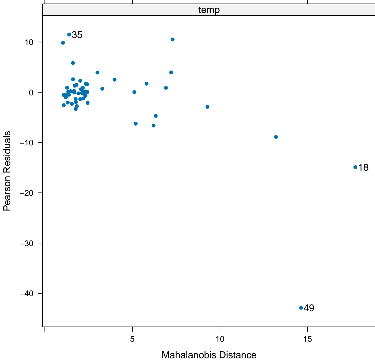
Pearson Residuals vs. Mahalanobis Distance
