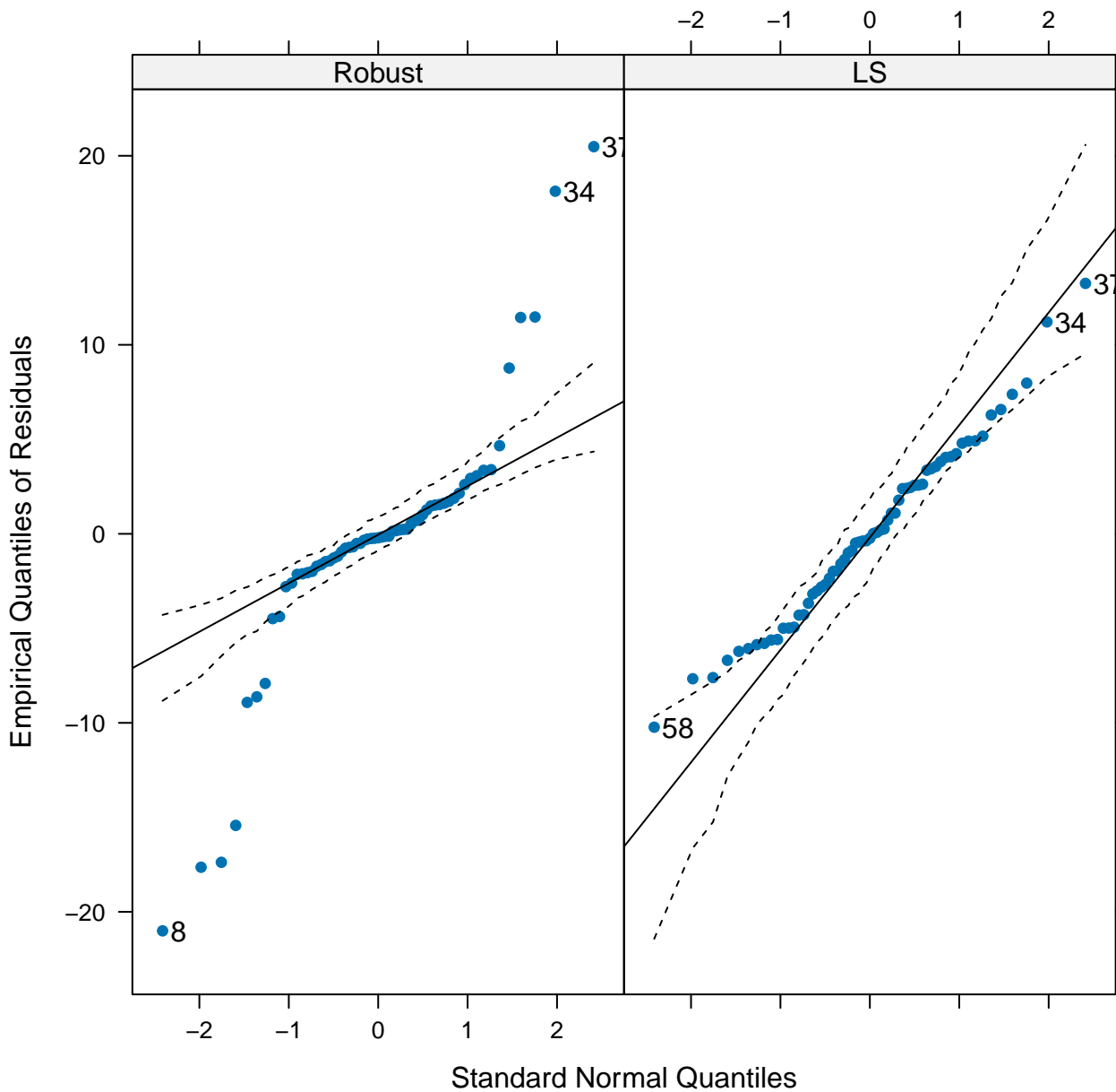
Normal QQ Plot of Residuals
