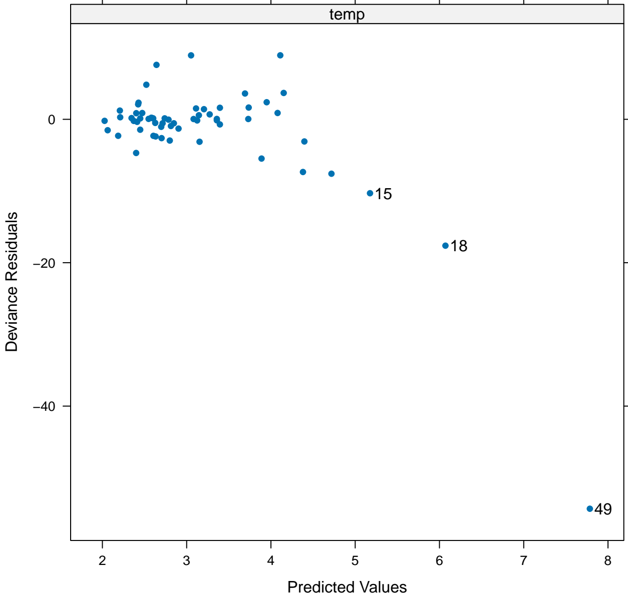
Deviance Residuals vs. Predicted Values
