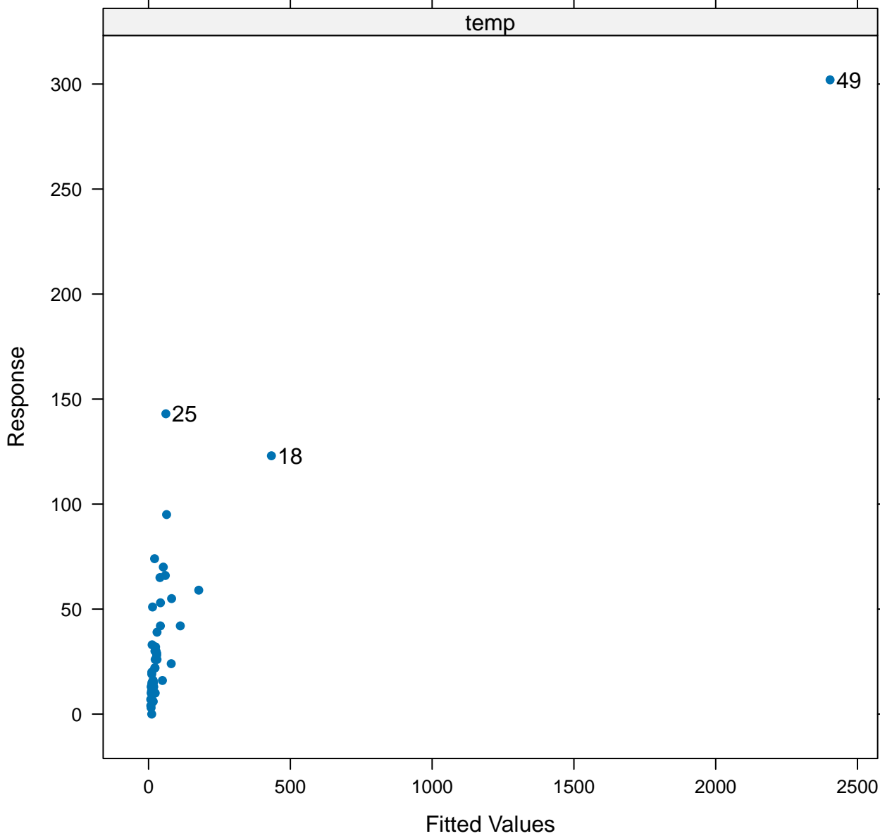
Response vs. Fitted Values
