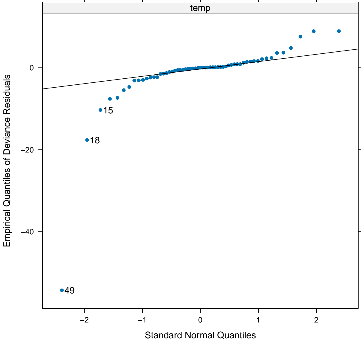
Normal QQ Plot of Deviance Residuals
