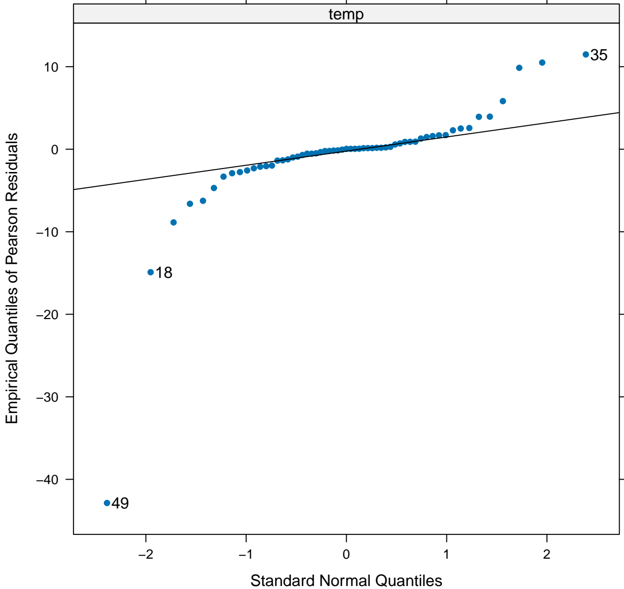
Normal QQ Plot of Pearson Residuals
