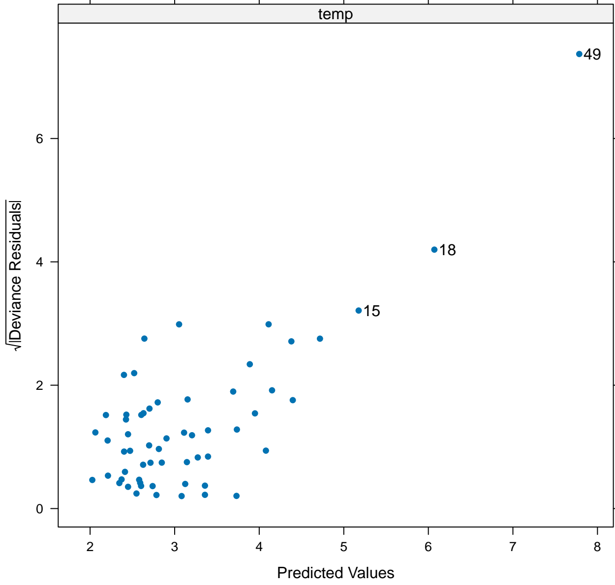
\sqrt{|\text{Deviance Residuals}|} vs. Predicted Values
