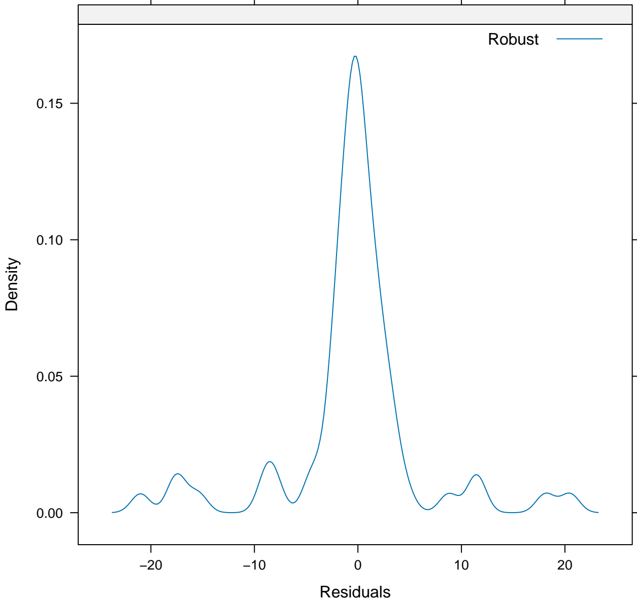
Kernel Density Estimate of Residuals
