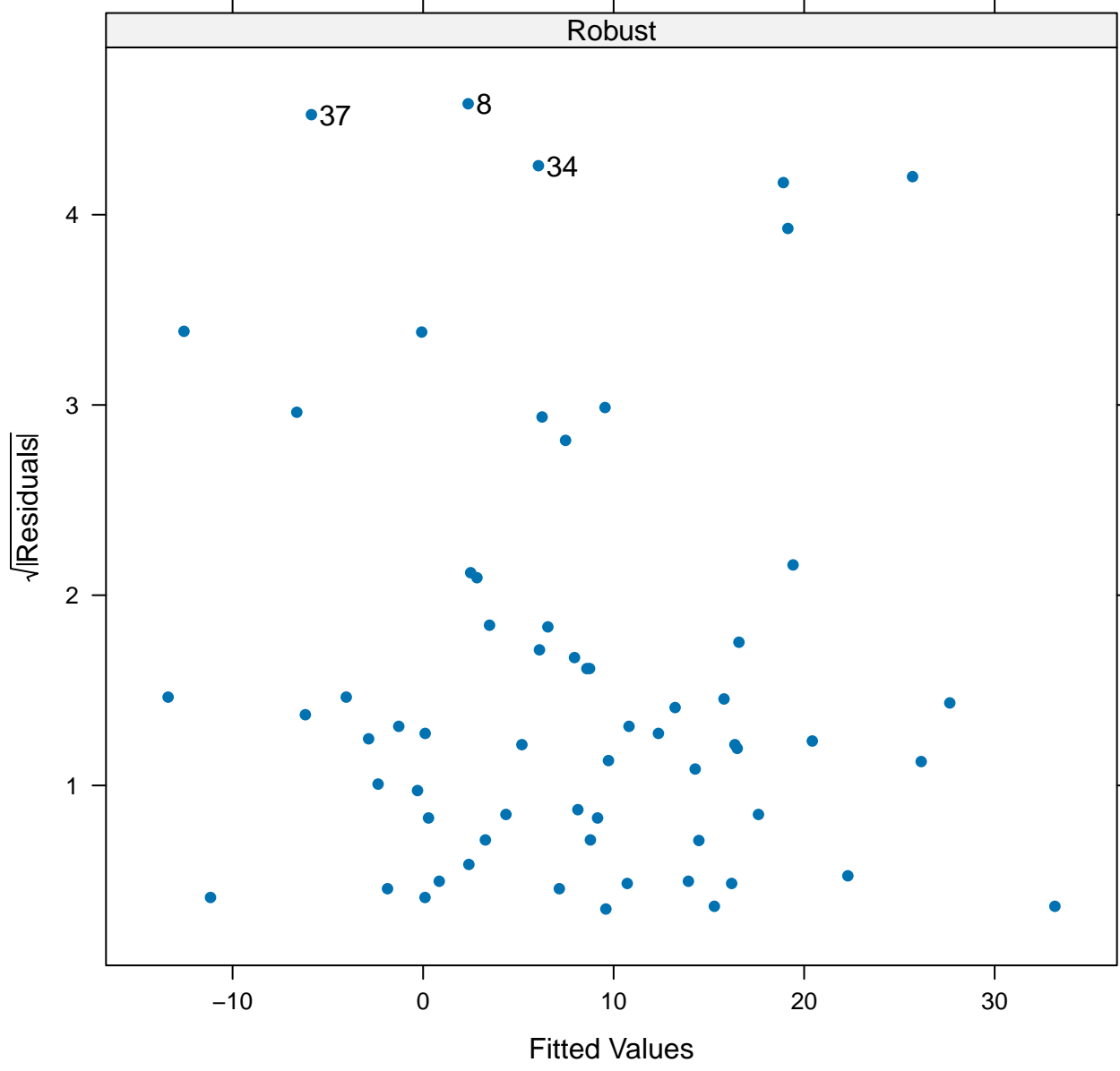
\sqrt{|\text{Residuals}|} vs. Fitted Values
