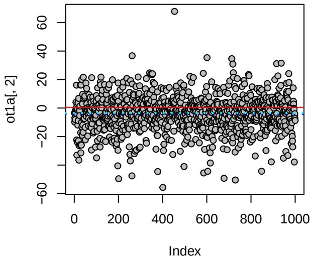
data A: estimated \gamma
