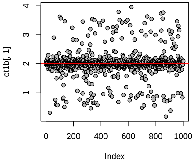
data B: estimated \beta
