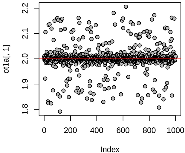
data A: estimated \beta
