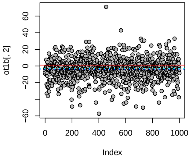
data B: estimated \gamma
