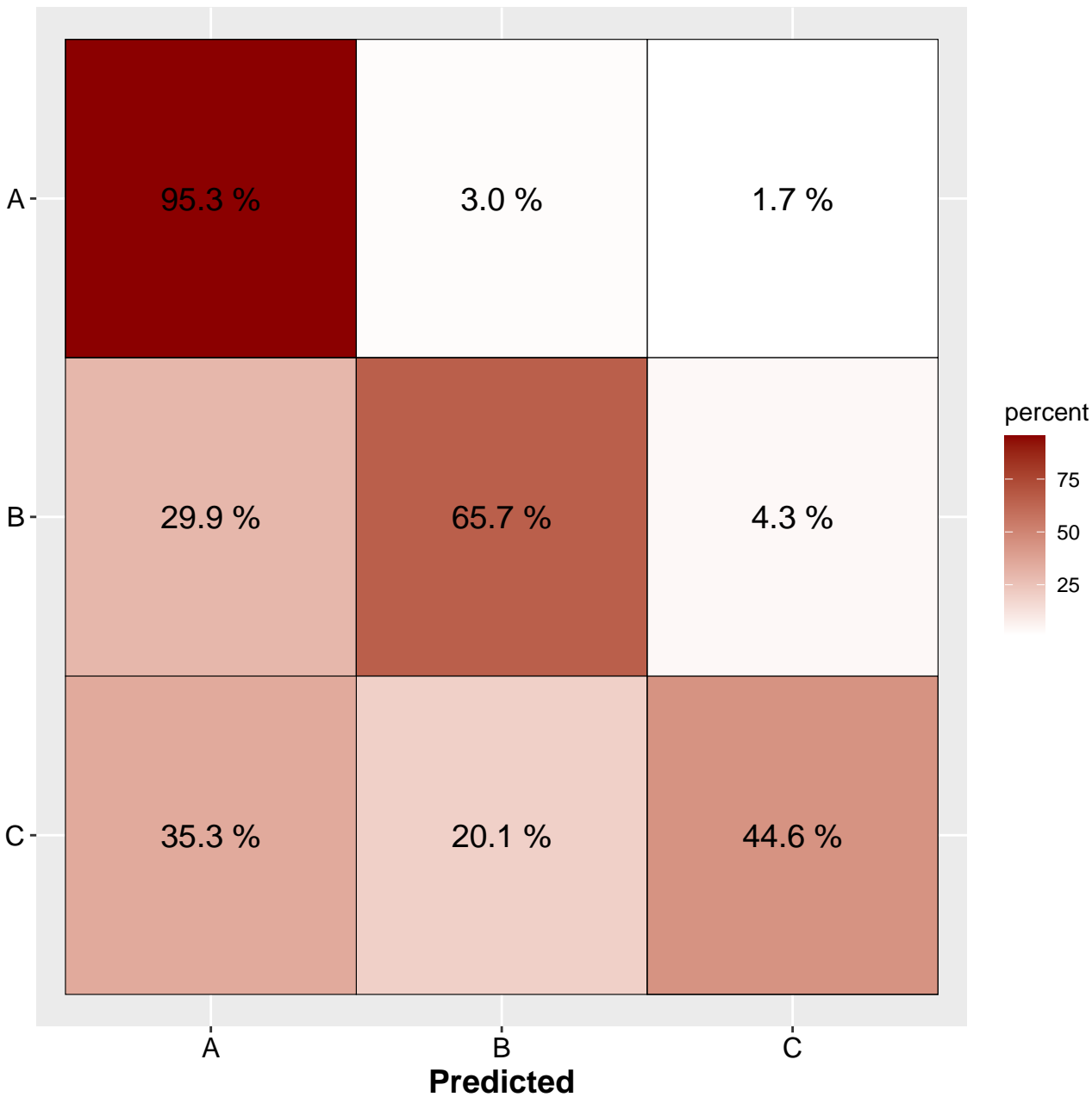
j48 performance on random features
