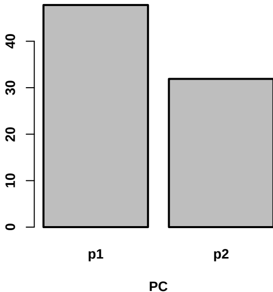
Scores (PCA)
