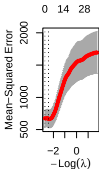
Group 4
