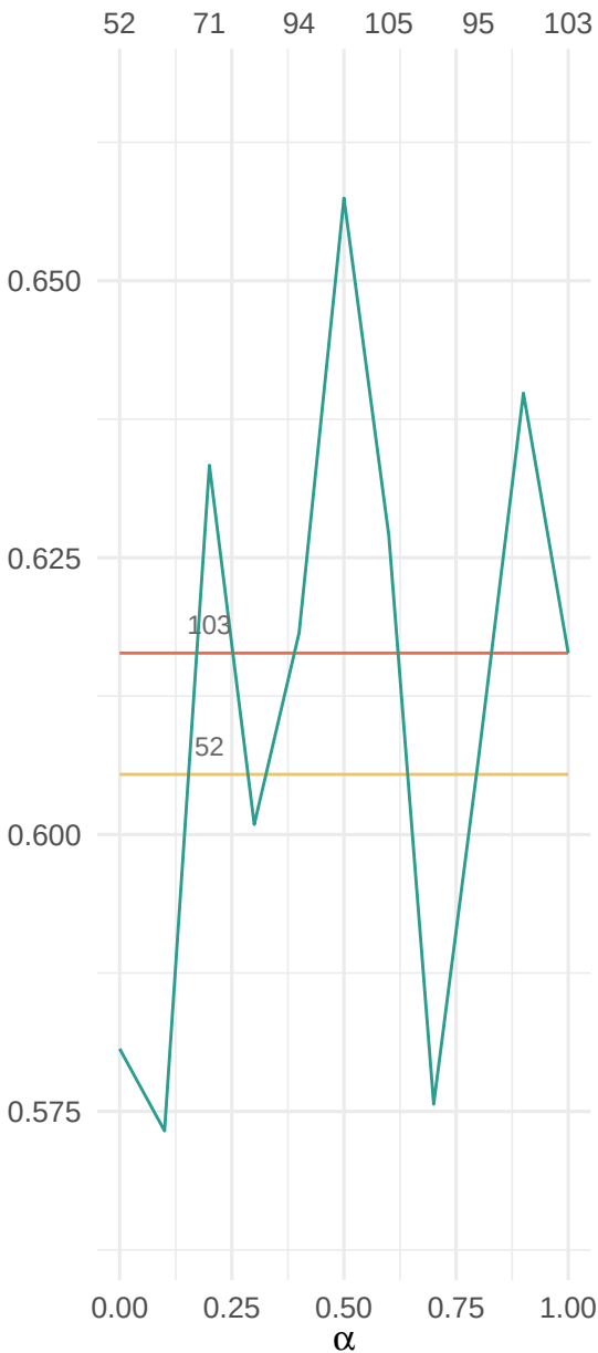
5 group problem
