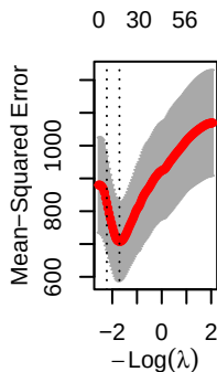
Group 3
