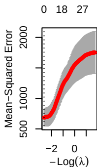
Group 4
