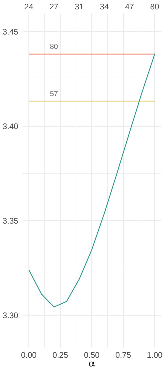
2 response problem
