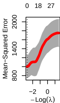
Group 5
