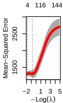
Group 1
