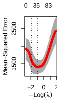
Group 1
