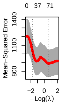
Group 2
