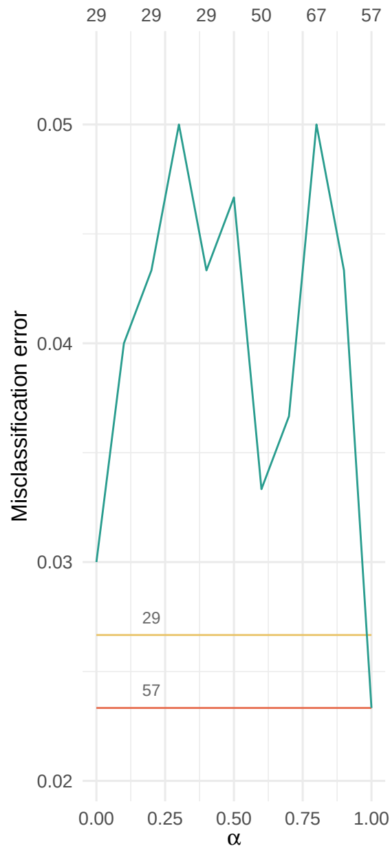
3 class problem
