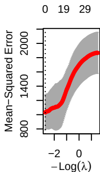
Group 5
