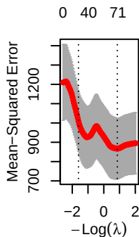
Group 2
