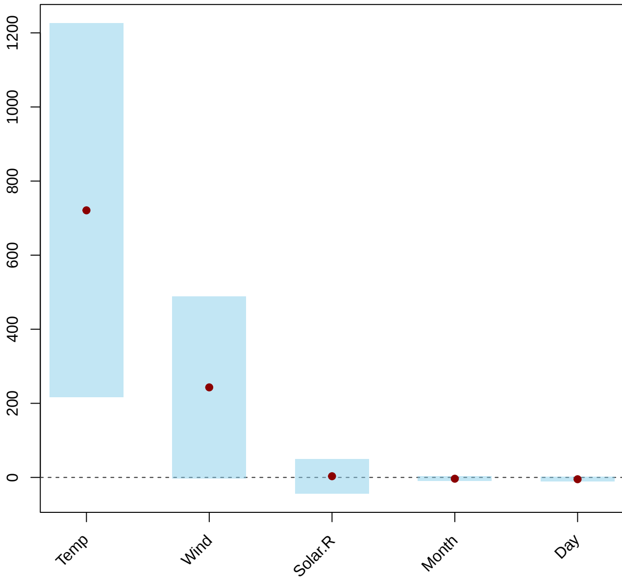
Conditional Permutation Importance (threshold = 0.95)
