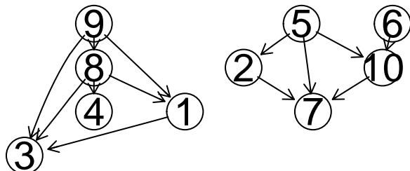
geometric
