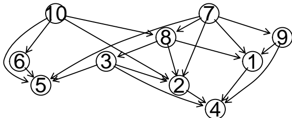
barabasi
