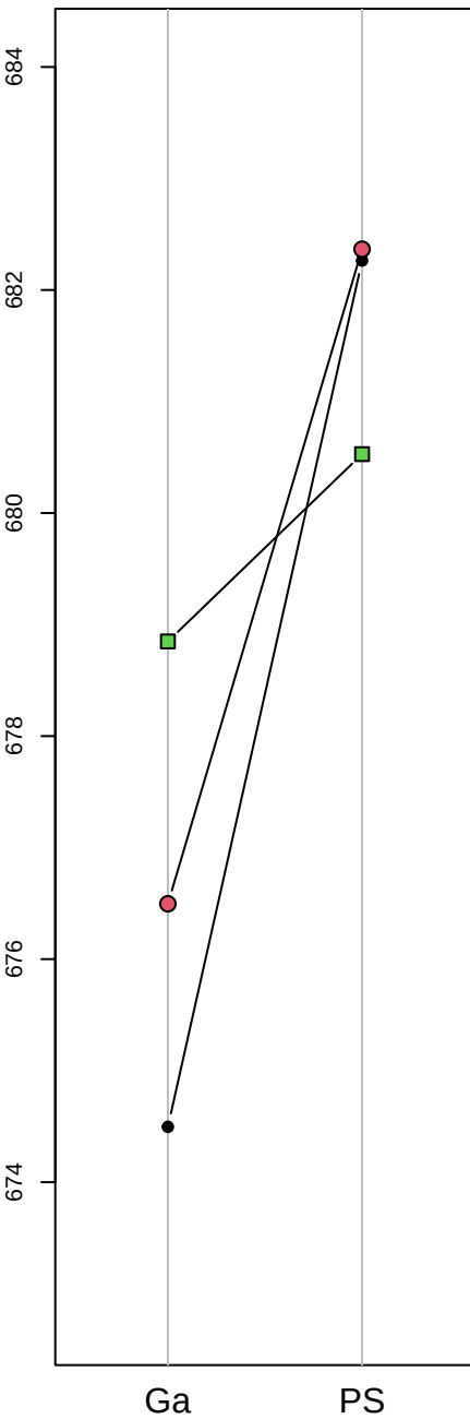
AIC
