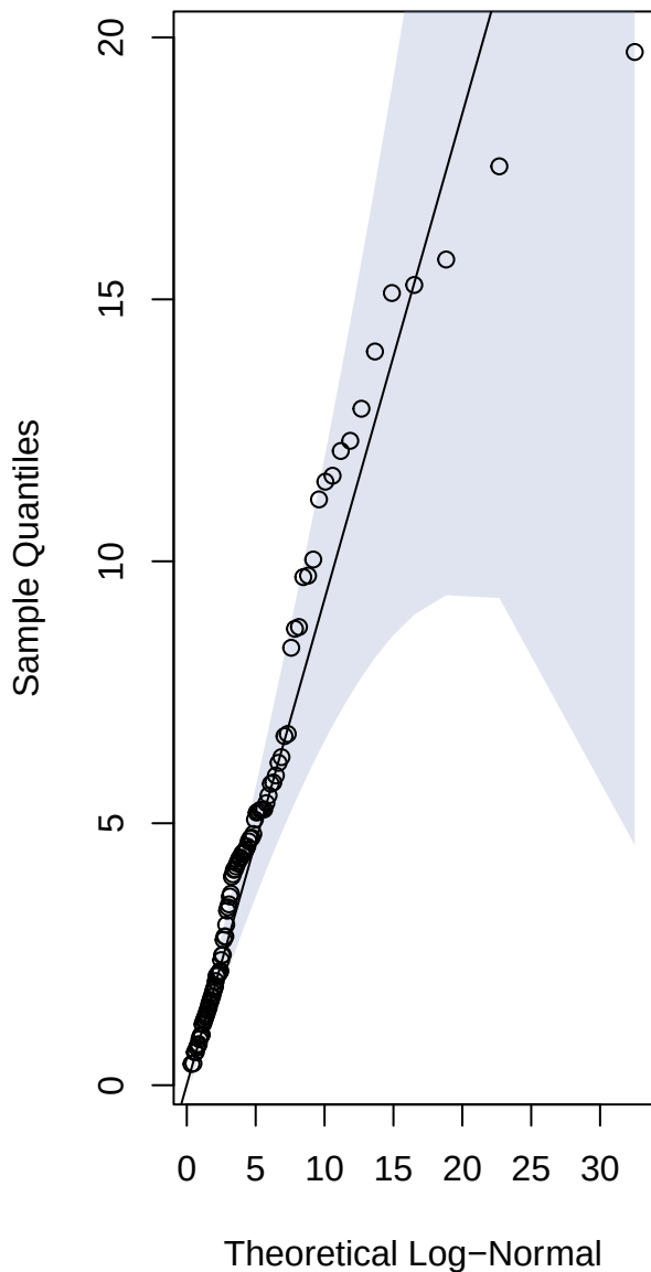
Biomarker (K-S : p = 0.8127 )
