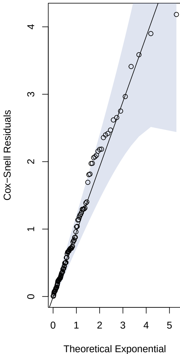
Time-to-event (K-S : p = 0.578 )
