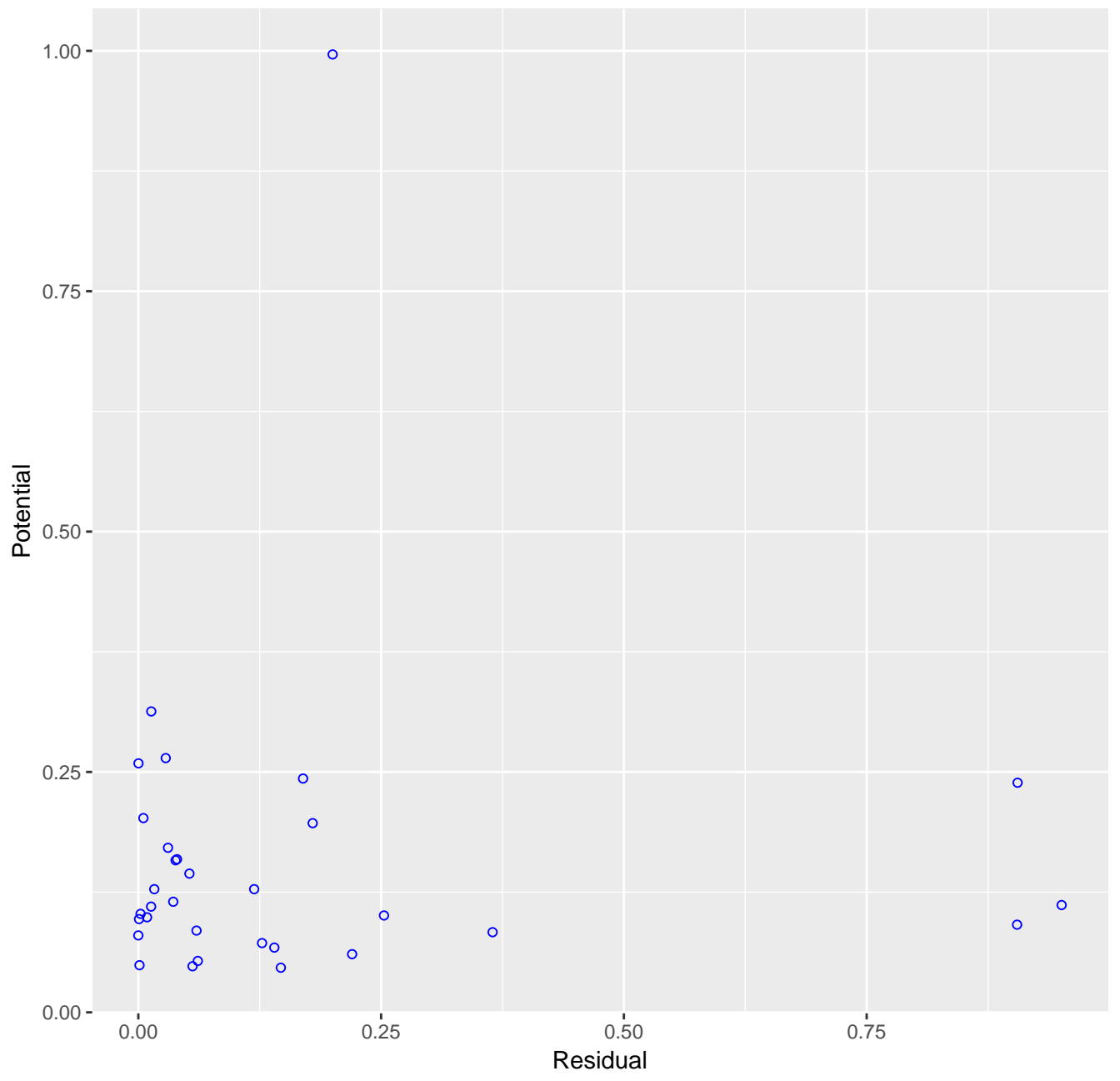
Potential-Residual Plot
