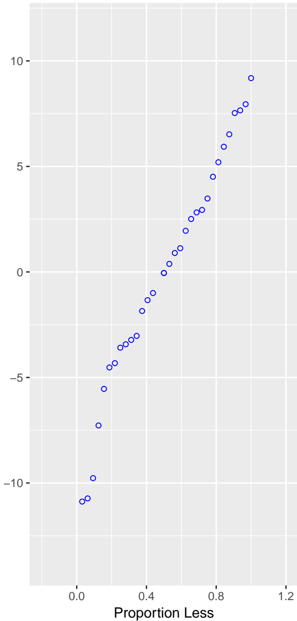
Fit – Mean
