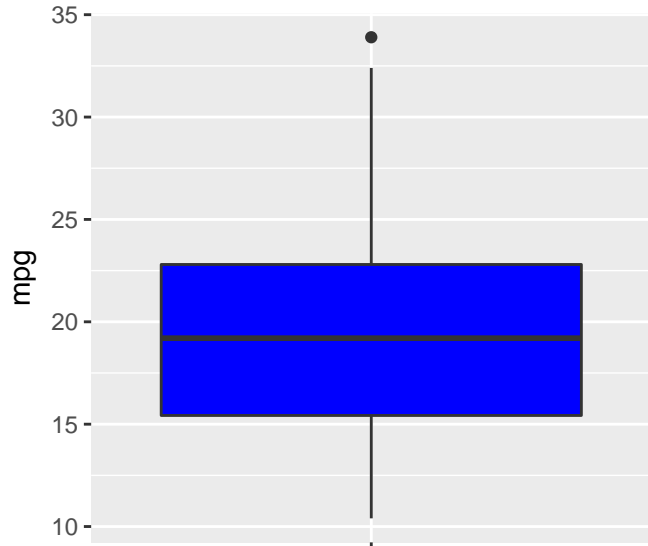
Boxplot of mpg
