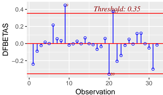
Influence Diagnostics for hp
