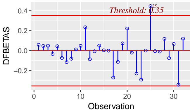
Influence Diagnostics for wt
