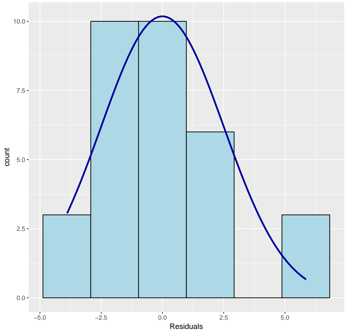
Residual Histogram
