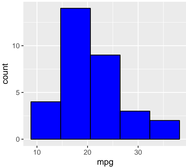
Histogram of mpg
