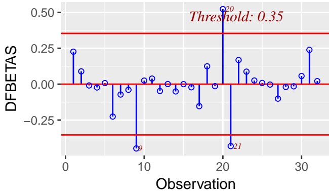
Influence Diagnostics for qsec
