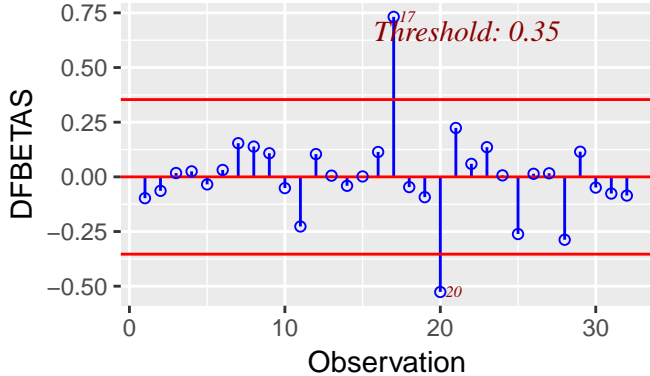
Influence Diagnostics for wt
