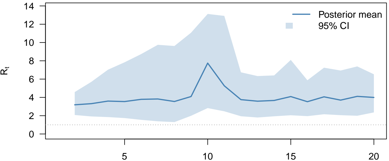
Effective reproduction number
