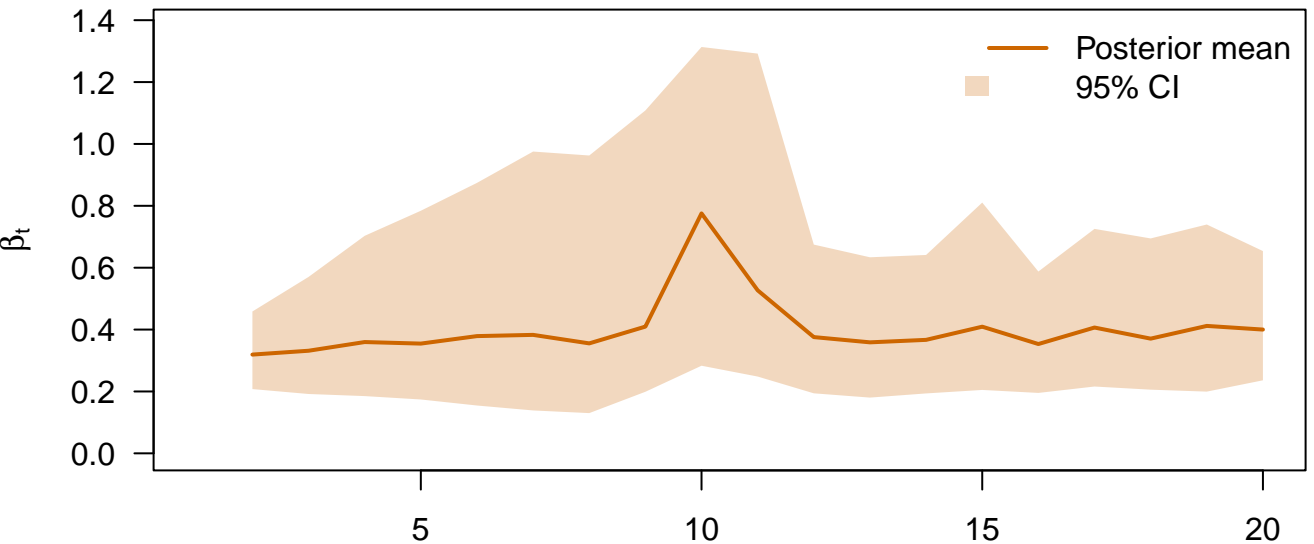
Transmission rate \beta_t
