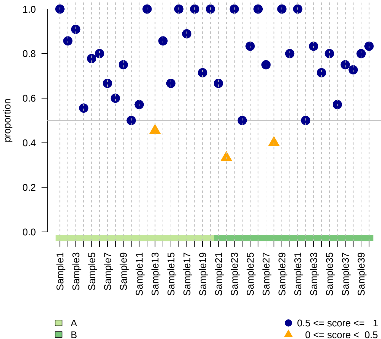
Freq. of being correctly classified (randomForest, 5 feat.)
