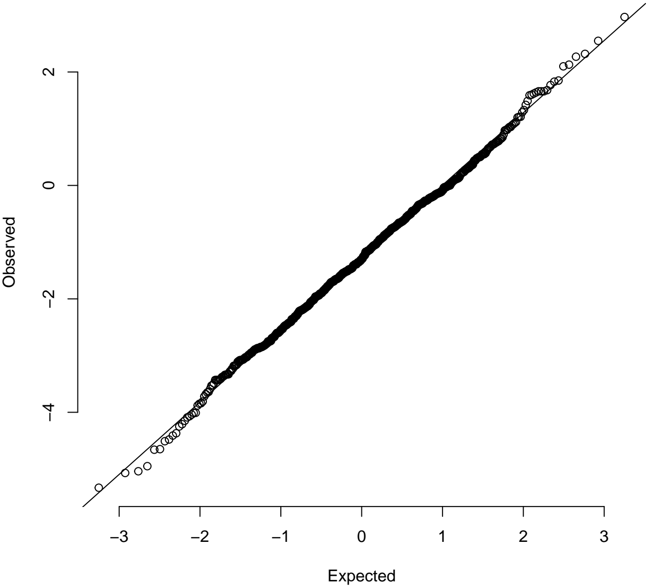
Normal Q-Q plot for svy$waz
