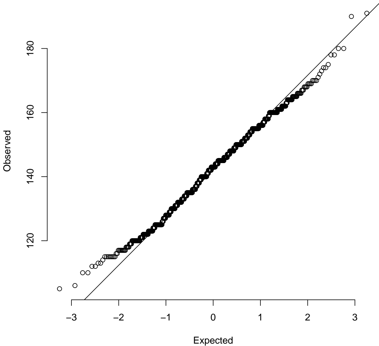
Normal Q-Q plot for svy$muac
