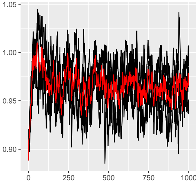
fixed effect 3
