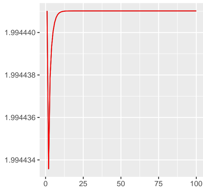
fixed effect 2
