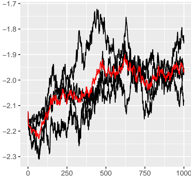
fixed effect 3
