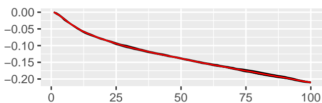
theta_K6
