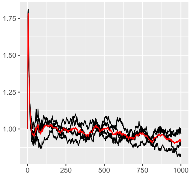
fixed effect 2
