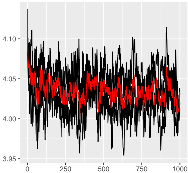
fixed effect 2
