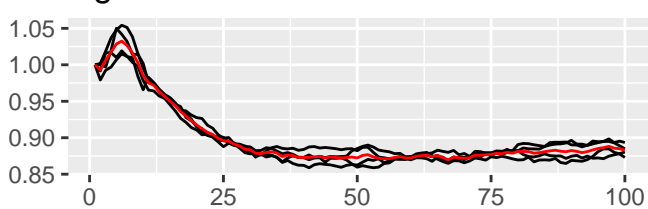
sigma
