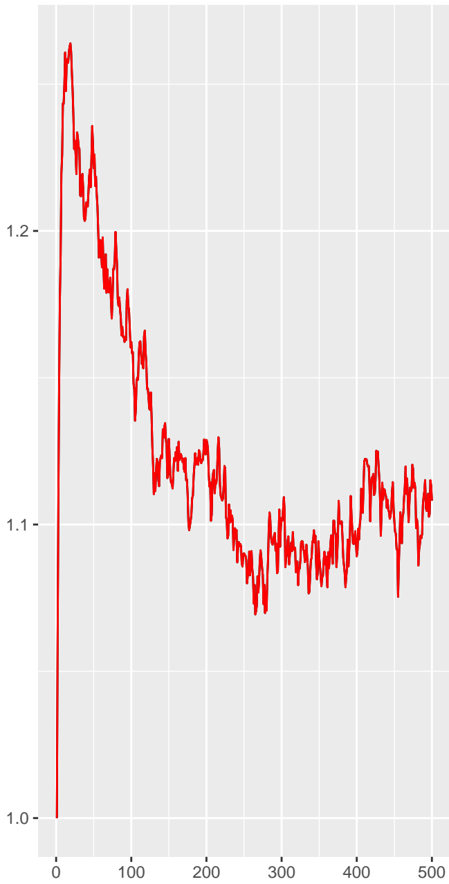
sigma
