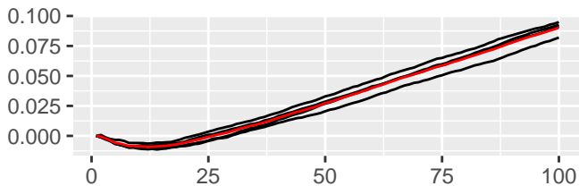
theta_K5
