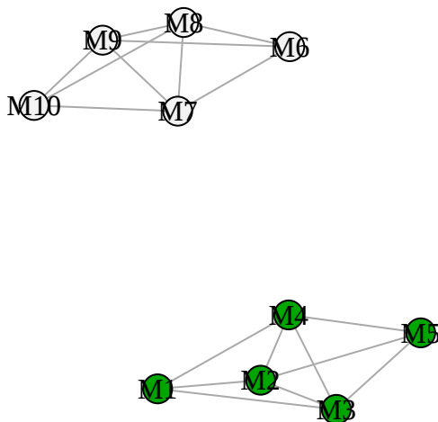
Graph structure
