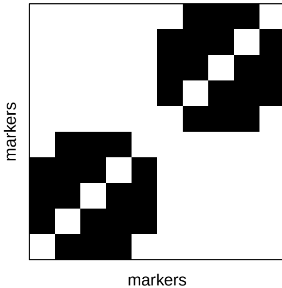
Adjacency Matrix
