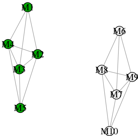
Graph structure
