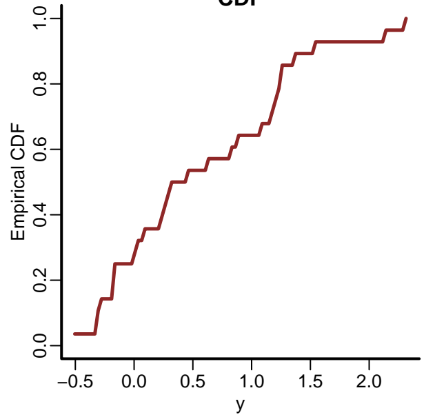
CDF
